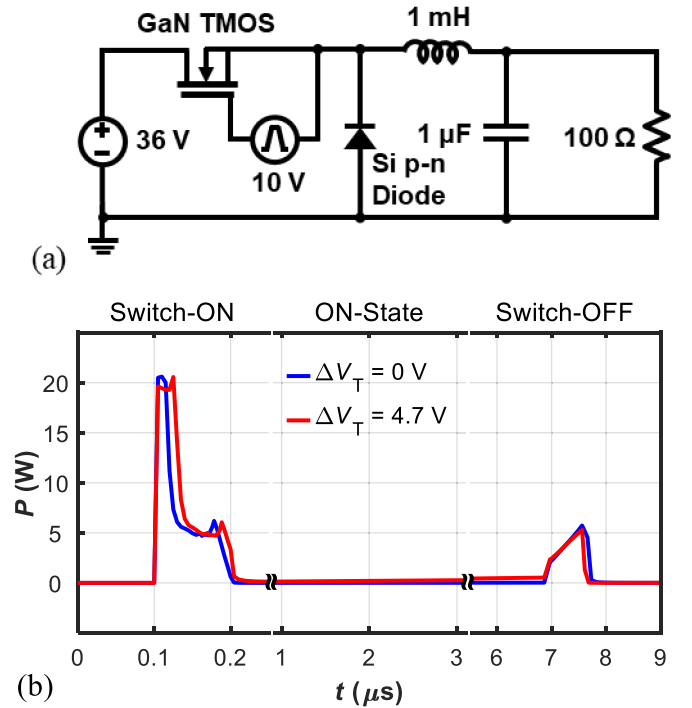
Fig. 11. (a) Circuit schematic of the simulated 36-12 V buck converter. (b) Simulated dissipated power by the TMOS during switch-ON, ON-state, and switch-OFF. Switching period is 20 \mu s . The origin on the x -axis corresponds to 3 ms, i.e., after 150 cycles from simulation start to ensure switching regime conditions are reached. The two curves correspond to the fresh TMOS (blue line) and the stressed TMOS with increased V_T (red curve) of 4.7 V, corresponding to the worst-case as obtained from experimental data in Fig. 4(a).
