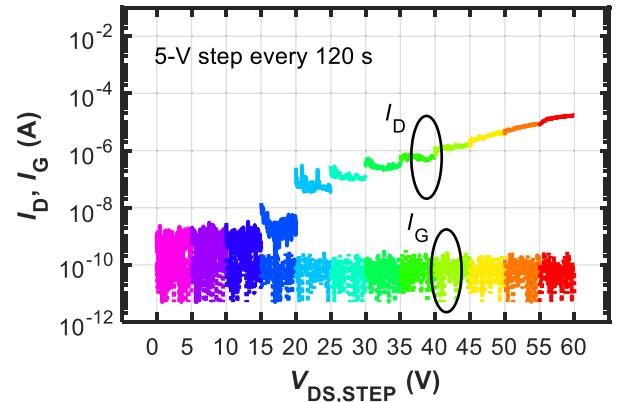
Fig. 6. Drain and gate leakage current during the step-stress experiment.
