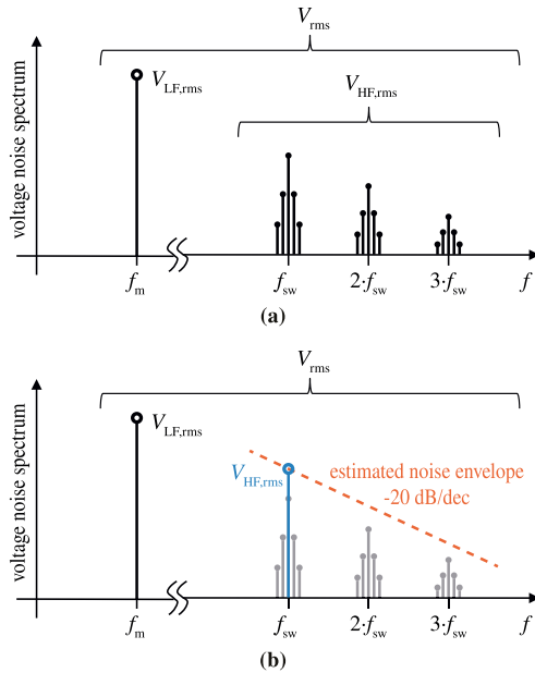
Fig. 3. (a) Typical rms spectrum of a switched voltage waveform including an LF fundamental component (frequency f_m ) V_{LF,rms} and HF harmonics V_{HF,rms} at integer multiples of the switching frequency (side bands). (b) Simplified noise estimation method presented in [24] for single-phase converters: all HF rms noise energy is concentrated in a lumped/single harmonic V_{HF,rms} at the switching frequency f_{sw} and an envelope with a slope of -20 dB/dec is used for estimating noise levels for f > f_{sw} .
