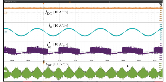
Fig. 11. Measurement results when operating the demonstrator from [16] at a 400 V mains with reduced CM SVPWM [27], an output voltage of 400 V, an output power of 10 kW, and a switching frequency of 100 kHz. In addition to the dc-link current, I_{DC} , the (filtered) input current of phase a, i_a , the switched transistor current i'_{ap} [see also Fig. 7(a)] and the voltage v_{nk} are shown. Similarly, the currents i'_{an} and the voltage v_{pk} are measured (not shown), which allows to calculate v_{DM,HF} from (13) and v_{CM} from (14). Note a small phase shift between i_a and i'_{ap} due to the capacitive current flowing through the first-stage filter capacitors. The key specifications of this hardware demonstrator are listed in Table II.
