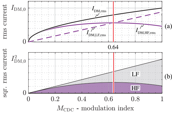
Fig. 9. (a) Analytical HF and LF DM rms currents of a 3- \Phi current dc-link PFC rectifier interfacing a 400 V mains with varying modulation indices M_{\text{CDC}} while maintaining a constant dc-link current of I_{\text{DC}} to supply different DC output voltages. (b) Breakdowns of the total squared rms DM currents generated by the switching stage, i.e., the LF and HF components with different modulation indices M_{\text{CDC}} . Note that a maximum HF DM rms current is observed when M_{\text{CDC}} = 2/\pi = 0.64 (solid red line).
