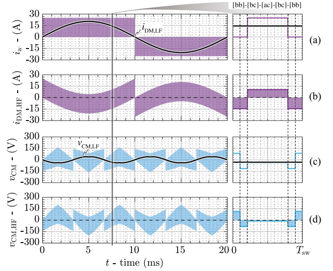
Fig. 8. Simulated key waveforms (with a zoomed view over one switching period) of the 3- \Phi current dc-link PFC rectifier [see Fig. 7(a)] operating with reduced CM SVPWM from a 400 V (line-to-line rms) mains with 400 V DC output voltage, 10 kW output power, and a dc-link current of 25 A. Taking phase a as an example, (a) shows the total DM input current i'_a , and (b) its HF component i'_{DM,HF} ; (c) shows the total CM noise voltage v_{CM} and (d) its HF component v_{CM,HF} , i.e., (b) and (d) indicate the pre-filter DM and CM noise emissions.
