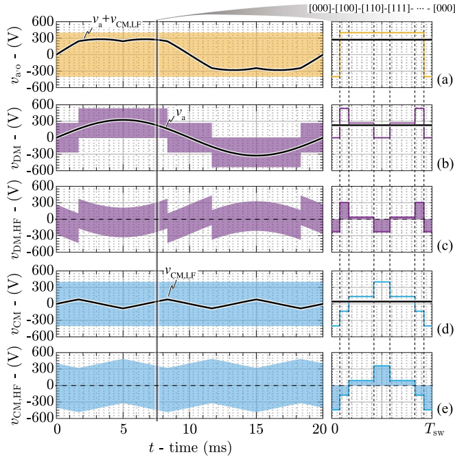
Fig. 2. Simulated key waveforms (with a zoomed view over one switching period) of the two-level 3- \Phi voltage dc-link PFC rectifier [see Fig. 1(a)] operating with a 400 V (line-to-line rms) mains, 800 V dc-link and/or output voltage, and 10 kW output power using the standard SVPWM. Taking phase a as an example, (a) shows the switching stage phase voltage v_{a'o} , which can be decomposed into (b) DM and (e) CM components. Furthermore, (c) and (f) show the DM and CM HF noise voltages (i.e., the pre-filter DM and CM noise emissions). Note that a typical symmetric switching sequence, i.e., mirrored with respect to the center of a switching period or the switching state [111] in the selected sector, is applied, and only the first half over one switching period is shown on top.
