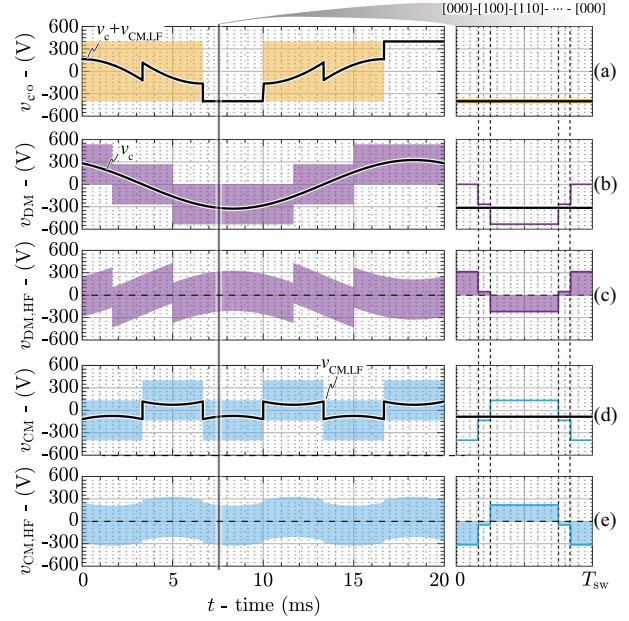
Fig. 15. Simulated key waveforms (with a zoomed view over one switching period) of the two-level 3- \Phi voltage dc-link PFC rectifier [see Fig. 1(a)] operating with a 400 V (line-to-line rms) mains, 800 V dc-link and/or output voltage, and 10 kW output power using discontinuous SVPWM (DPWM). Taking phase c as an example, (a) shows the switching stage phase voltage v_{c-o} , which can be decomposed into (b) DM and (c) CM components. Furthermore, (c) and (f) show the DM and CM HF noise voltages (i.e., the pre-filter DM and CM noise emissions). Note that the phase with the maximum absolute voltage, i.e., phase c in the selected sector, is clamped during the entire sector, which is achieved by a suitable LF CM injection v_{\text{CM,LF}} , and hence the corresponding bridge leg is not switching within the switching period (only the first half of one switching period is shown in the zoomed view due to the switching sequence symmetry).
