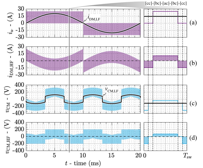
Fig. 17. Simulated key waveforms (with a zoomed view over one switching period) of the 3- \Phi current dc-link PFC rectifier [see Fig. 7(a)] operating with the conventional SVPWM, i.e., using the phase with the maximum absolute voltage as the zero state instead of the phase with the minimum absolute voltage in the RCM SPWM (see Fig. 8), from a 400 V (line-to-line rms) mains with 400 V DC output voltage, 10 kW output power, and a dc-link current of 25 A. Taking phase a as an example, (a) shows the total DM input current i_a and (b) its HF component i_{DM, HF} ; (c) shows the total CM noise voltage v_{CM} and (d) its HF component v_{CM, HF} .
