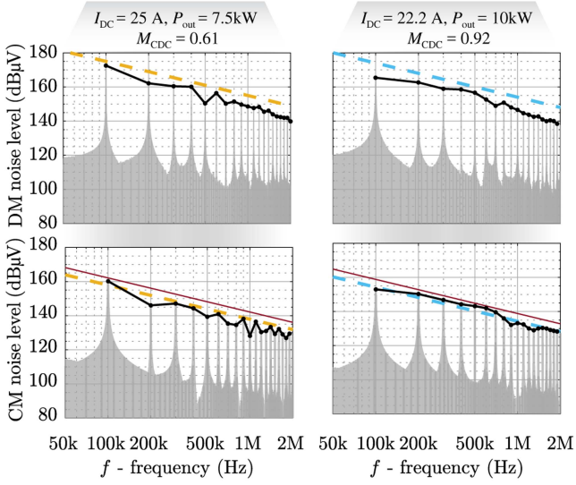
Fig. 18. DM (top row) and CM (bottom row) pre-filter noise amplitude spectra (the black solid lines indicate the envelopes of the measured spectra) extracted from circuit simulations of a 10 kW 3- \Phi current dc-link PFC rectifier modulated by the conventional SVPWM. The rectifier interfaces a 400 V mains using a switching frequency of 100 kHz with different modulation indices M_{\text{CDC}} (i.e., different power levels). The envelopes (dashed) are obtained with the low-complexity analytical expressions (16) for DM and (21) for CM, respectively as derived in Section III-A for the RCM SVPWM, which are grouped by colors according to the respective operating points. As a comparison, the CM noise envelopes specifically derived for the conventional SVPWM in Appendix D are shown as red solid lines; the DM noise envelopes are identical for both PWM schemes.
