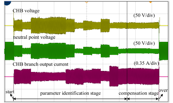
Fig. 17. Waveforms of experimental under neutral point ungrounded.
