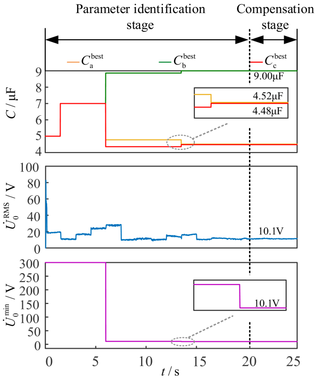
Fig. 12. Iteration process of algorithm parameters ( C_{0a} = 4.54 \mu\text{F} , C_{0b} = 8.86 \mu\text{F} , and C_{0c} = 4.56 \mu\text{F} ).
