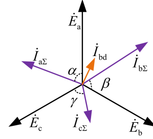
Fig. 2. Current relationship diagram.
