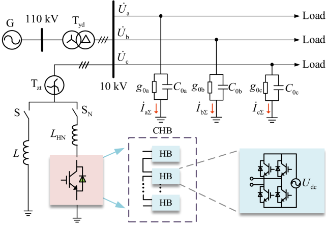
Fig. 1. Structure of the neutral point connected with the active compensation device.
