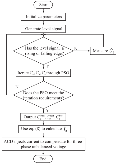
Fig. 5. Flowchart of the proposed strategy.
