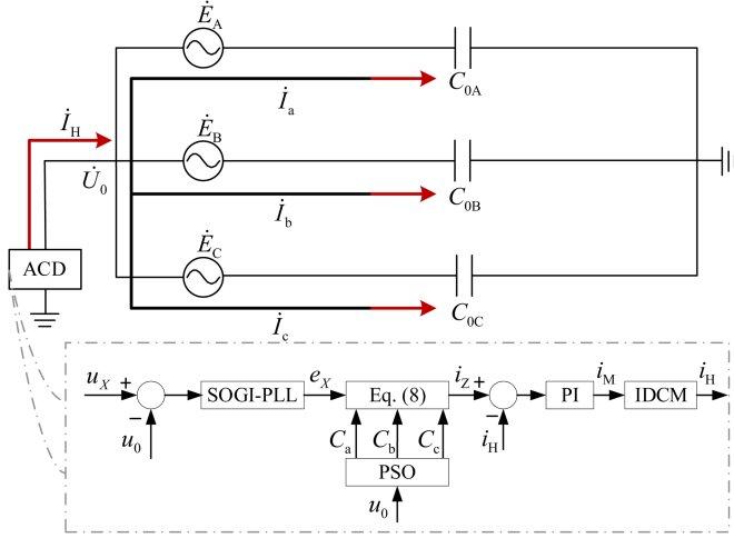
Fig. 4. Asymmetrical structure of phase-to-ground parameters of the distribution network.
