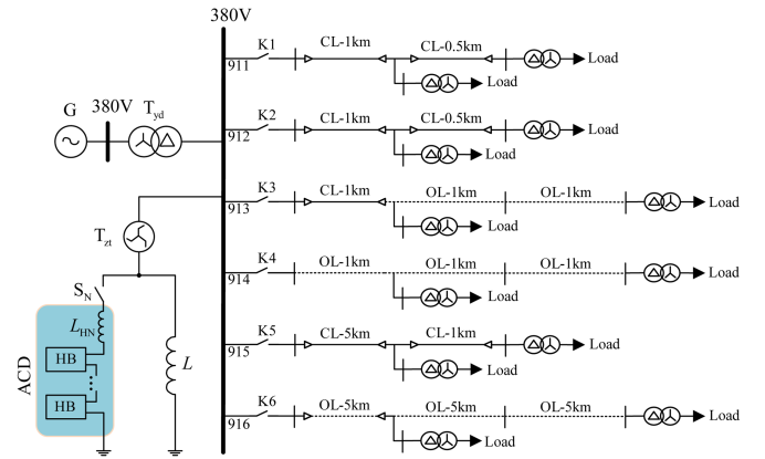
Fig. 10. Single-line diagram of the experimental setup.
