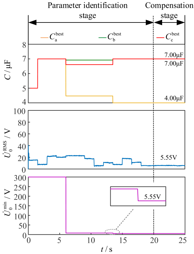
Fig. 15. Iteration process of algorithm parameters ( C_{0a} = 4.32 \mu\text{F} , C_{0b} = 6.89 \mu\text{F} , and C_{0c} = 6.94 \mu\text{F} ).
