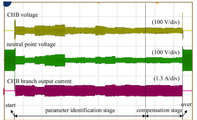
Fig. 14. Waveforms of experimental under neutral point grounded through arc suppression coil.
