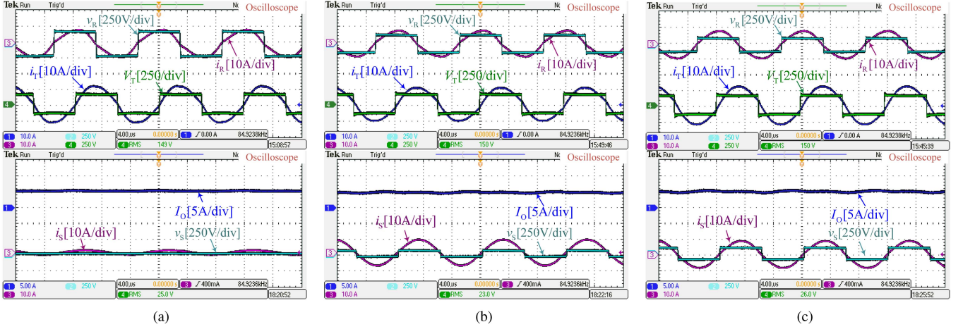
Fig. 18. Experimental waveforms of the proposed IPT charging system with RSP at various misalignment conditions: (a) \Delta X = 0 mm (fully aligned). (b) \Delta X = 50 mm. (c) \Delta X = 100 mm. (a) \Delta X = 0 mm (fully aligned). (b) \Delta X = 50 mm. (c) \Delta X = 100 mm.
