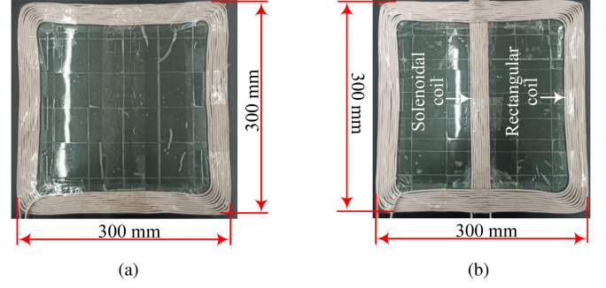
Fig. 12. Top view of the Tx rectangular coil pad and the Rx RSP. (a) Tx rectangular coil pad. (b) Rx RSP.
