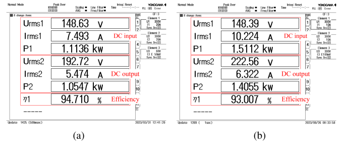
Fig. 20. Measured power efficiency at various misalignment conditions. (a) \Delta X = 0 mm. (b) \Delta X = 150 mm.
