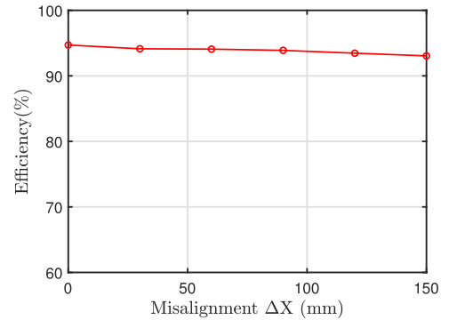
Fig. 21. Measured transfer efficiency of proposed IPT under different misalignments along the X-axis.
