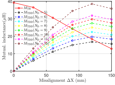
Fig. 10. Mutual inductances M_{TR} and M_{TDD} of the coupler with DDQP under various misalignments along X -axis versus N_D .
