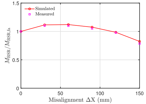
Fig. 17. Normalized mutual inductance M_{RSP} with N_S = 9 under different X-misalignments.
