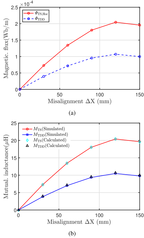
Fig. 7. (a) Numerically calculated results of the effective magnetic flux captured by the solenoidal coil and the DD coil ( \Phi_{TS,Hor} , \Phi_{TDD} ). (b) Corresponding mutual inductances versus misalignment distances along the X-axis direction.
