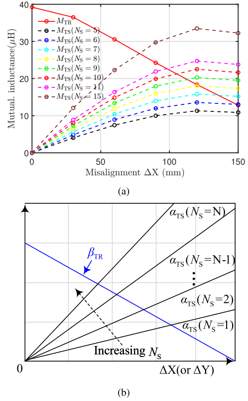
Fig. 8. (a) Mutual inductances M_{TR} and M_{TS} . (b) Approximate slope matching design principles of the proposed coupler with RSP under various misalignments along X-axis versus N_S .
