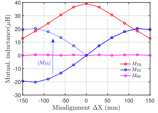
Fig. 13. Mutual inductance polarity of RSP coupler.
