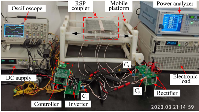
Fig. 15. Experimental prototype of 1-kW IPT system with RSP coupler.
