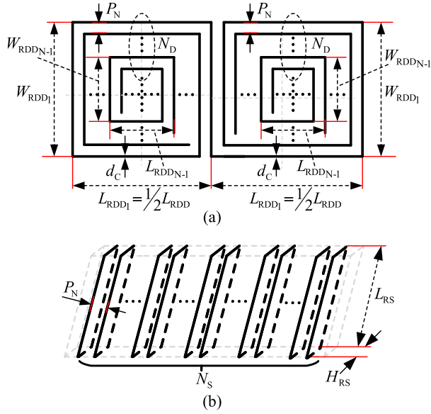
Fig. 6. Geometries of (a) solenoidal coil and (b) DD coil.
