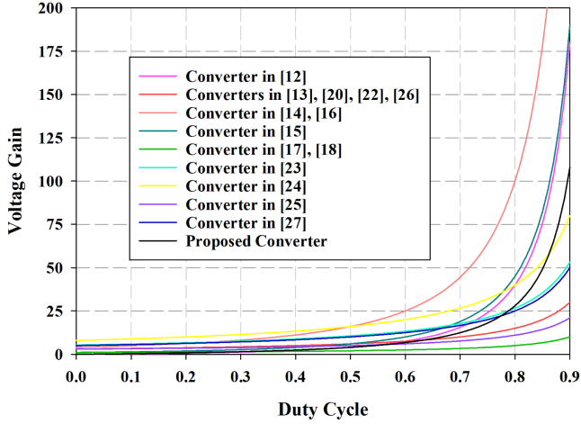
Fig. 5. Comparison of voltage gain: proposed converter versus other converters in [12], [13], [14], [15], [16], [17], [18], [20], [22], [23], [24], [25], [26], and [27] ( n = 1 and coupling factor ( k ) = 1).
