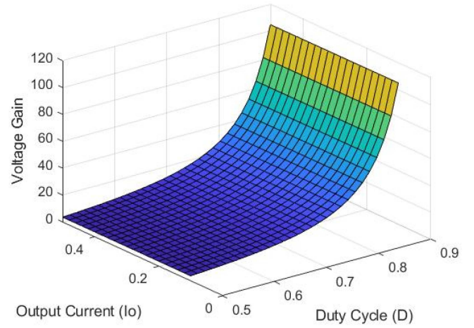
Fig. 7. Voltage gain ratio of the converter versus I_o and duty cycle ( D ) based on (31).
