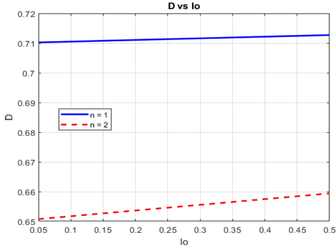
Fig. 6. Duty cycle versus output current for different turn ratios ( n ). Equation (28) is used to plot this graph, analyzing the effect of leakage inductance ( L_{lk1} ) when the output load changes.
