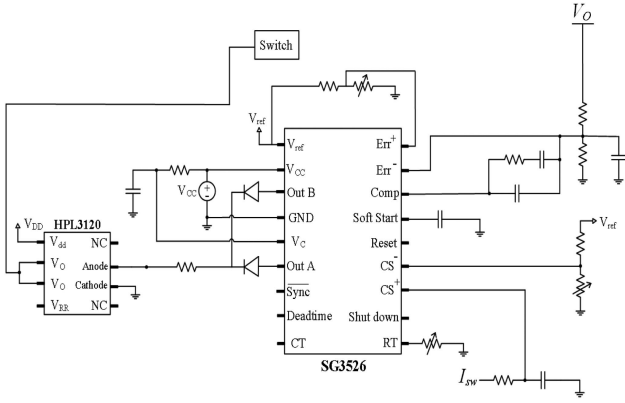
Fig. 13. Control circuit of the proposed converter.
