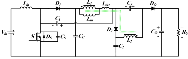
Fig. 2. Proposed soft-switched, single-switch high step-up converter.
