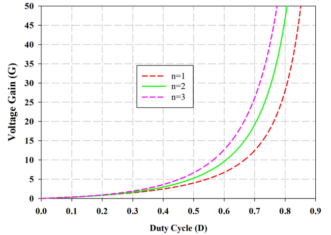
Fig. 8. Voltage gain ratio versus duty cycle for different turn ratios ( n ), without leakage inductance ( L_{lk1} ) (32).
