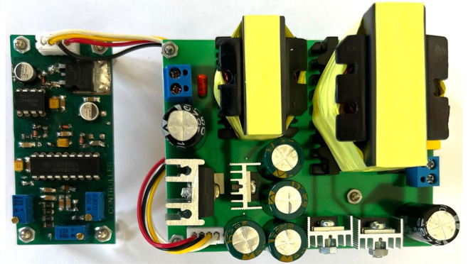
Fig. 12. Power and control prototype of the proposed converter.
