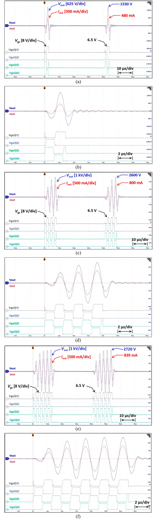
Fig. 7. Active cycle control by gate pulses V_{gs} for different duty cycles. (a) One cycle for 6.25% and partially zoomed in (b), (c) threecycles for 18.75% and partially zoomed in (d), (e) five cycles for 31.25% and partially zoomed in (f).
