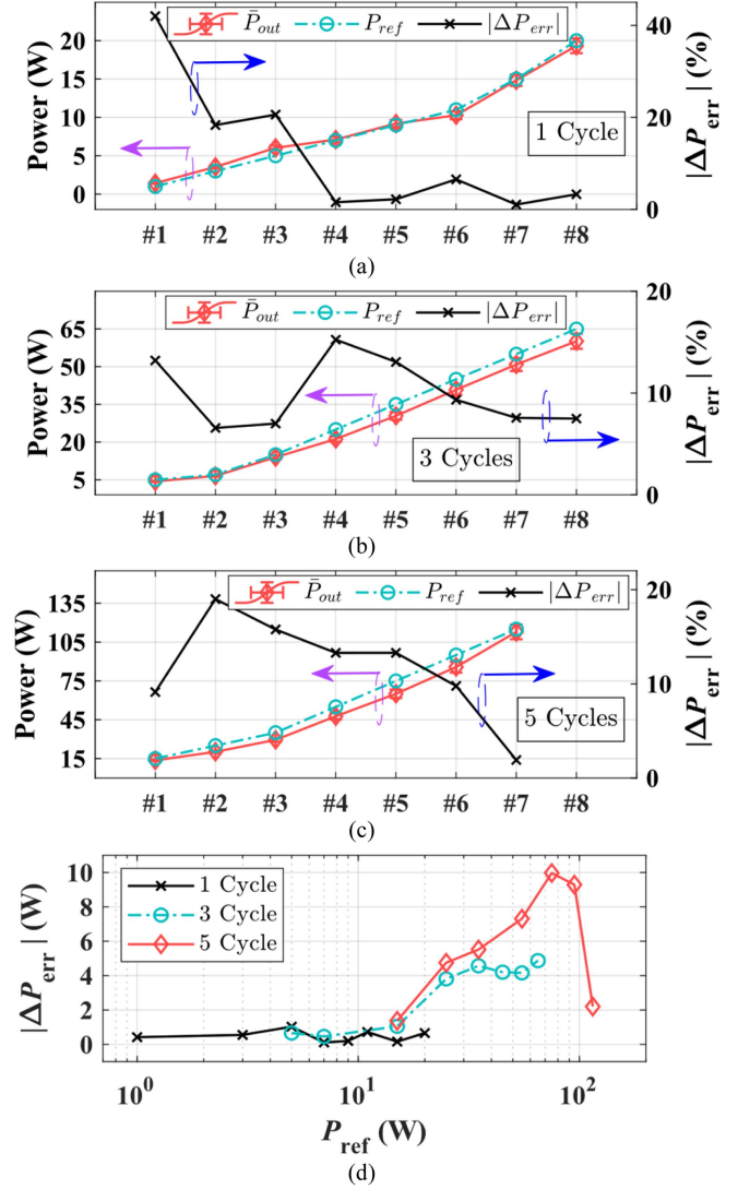
Fig. 14. Power tracking performance for biotissue load with (a) one active cycle, (b) three active cycles, (c) five active cycles, and (d) absolute value of tracking errors.
