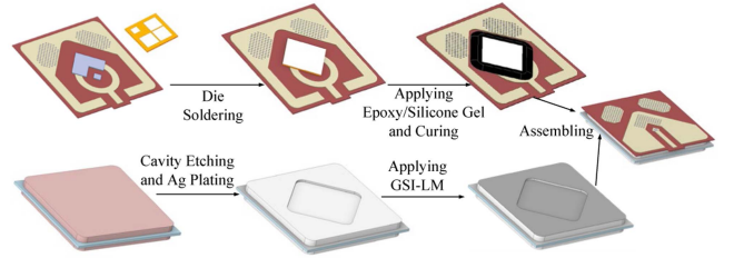
Fig. 7. Fabrication process of the GaInAg-LM FPCB/AMB hybrid packaging.
