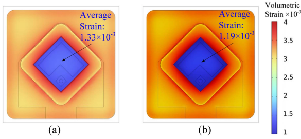
Fig. 4. Comparison of volumetric thermal strain of the die and AMB. (a) Solder-based packaging. (b) LM-based packaging.
