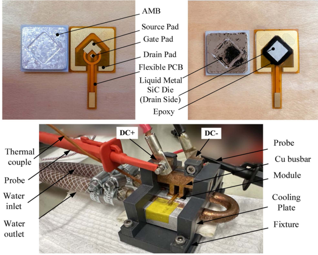
Fig. 8. Prototype of LM-based packaging and experimental setup.
