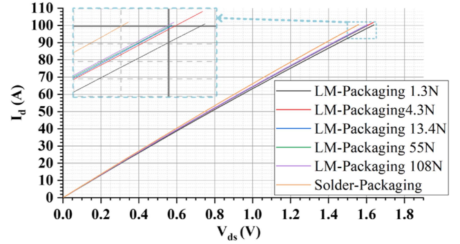
Fig. 10. Output characteristics comparison between solder packaging and LM packaging under different pressures ( V_{gs} = 18 V).
