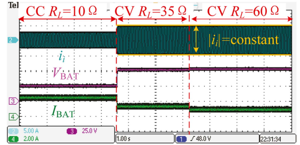
Fig. 12. Transient waveforms for R_L step changing from 10 to 35 Ω and from 35 to 60 Ω of the experimental prototype with SP-PS compensation as the IPT network and Ladder circuit 1 as the clamping network.
