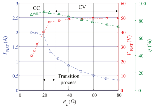
Fig. 11. Measured DC output current I_{BAT} , DC output voltage V_{BAT} , and power efficiency \eta versus load resistance R_L of the experimental prototype with SP-PS compensation as the IPT network and Ladder circuit 1 as the clamping network.
