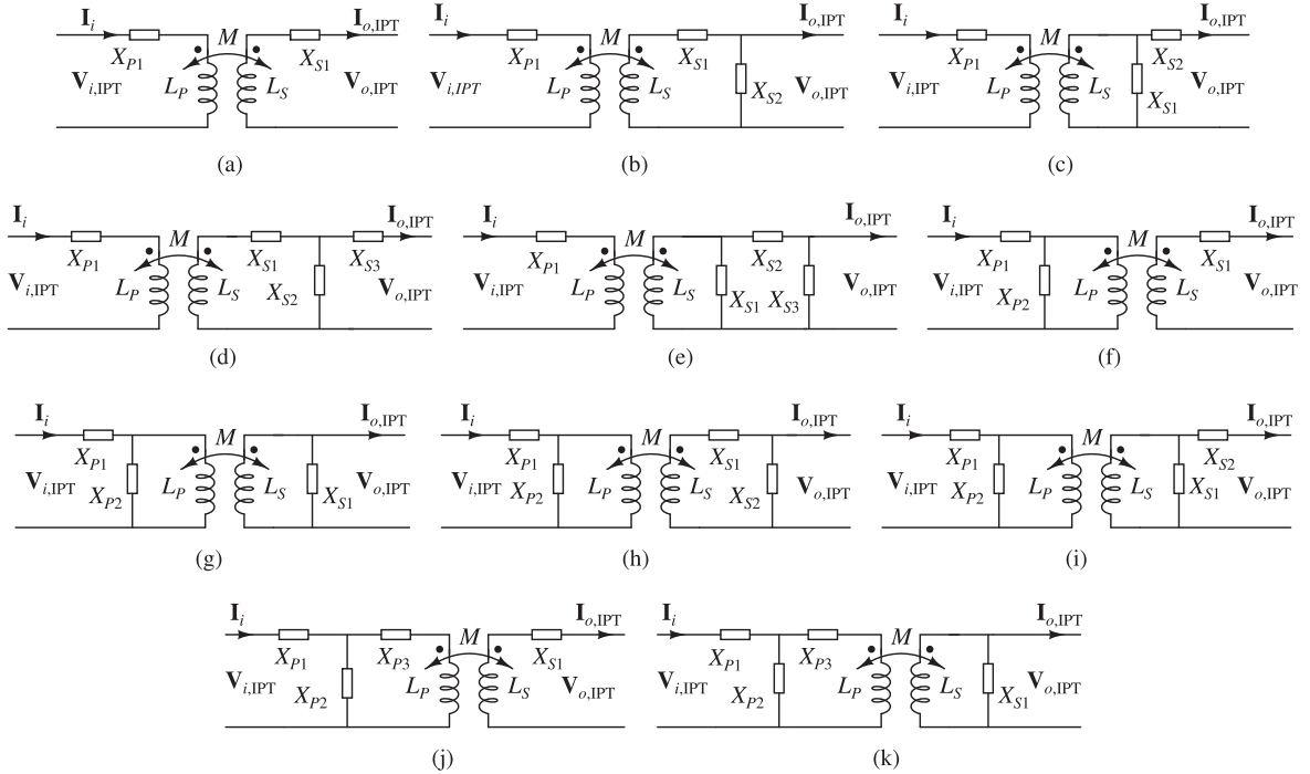
Fig. 3. Available IPT immittance networks with up to four compensation components. (a) S-S. (b) S-SP. (c) S-PS. (d) S-T. (e) S-II. (f) SP-S. (g) SP-P. (h) SP-SP. (i) SP-PS. (j) T-S. (k) T-P.
