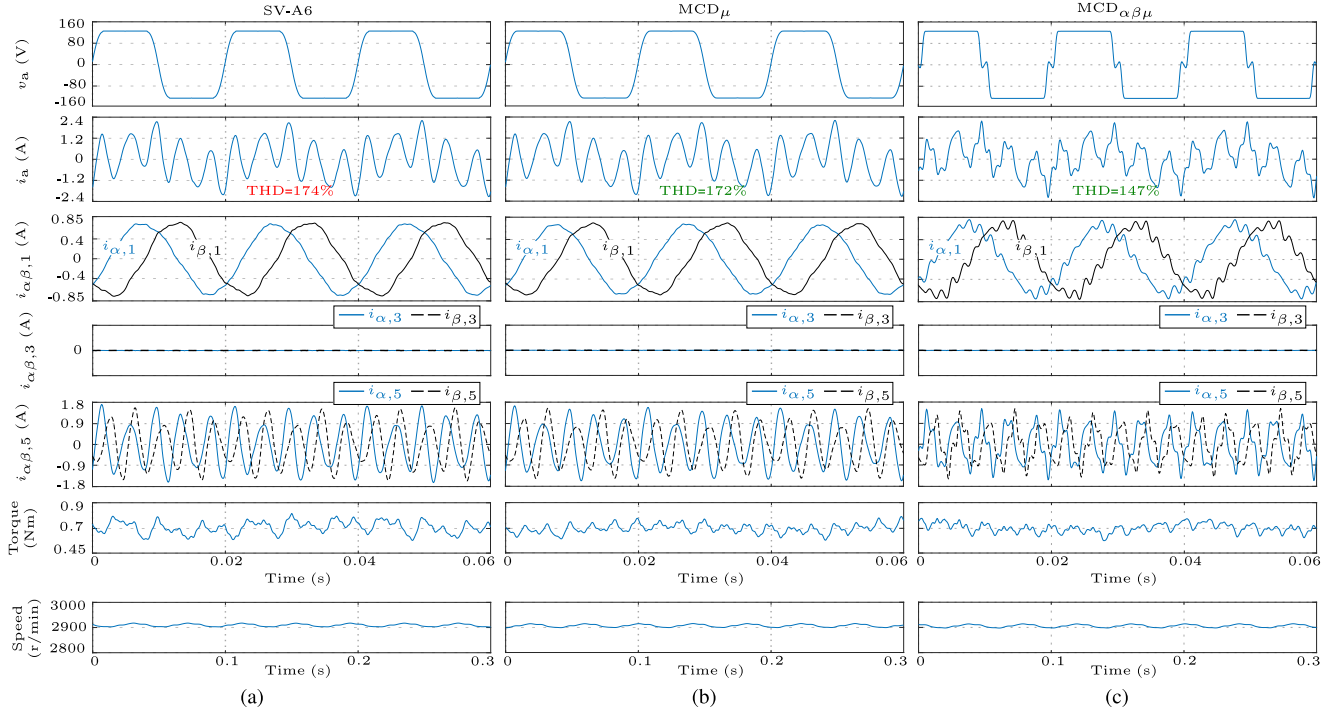
Fig. 15. Experimental results of A6N2 in the time domain of (a) SV-A6, (b) MCD_\mu , and (c) MCD_{\alpha\beta\mu} for M = 1.24 . From top to bottom: inverter pole-voltage reference of phase a v_a ; current of phase a i_a ; \alpha\beta_1 current; \alpha\beta_3 current; \alpha\beta_5 current; electromagnetic torque; and rotor speed.
