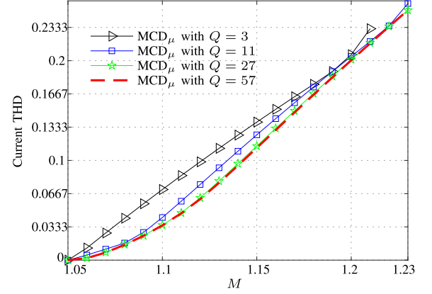
Fig. 2. Current THD (voltage WTHD) of \text{MCD}_\mu for S5N1.
