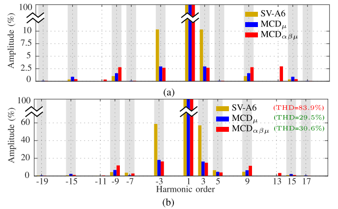
Fig. 14. Experimental spectra of A6N1 for M = 1.10 of the (a) phase-voltage references and (b) stator currents. The \alpha\beta_3 and \alpha\beta_5 harmonics are shaded.
