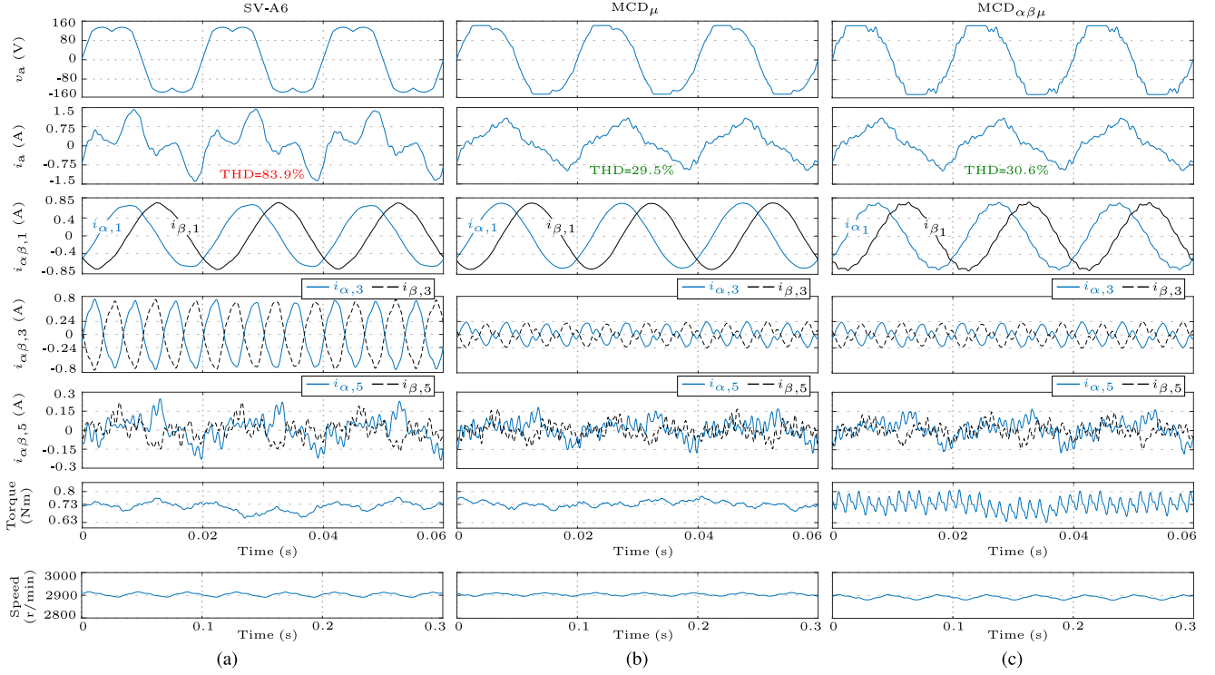
Fig. 13. Experimental results of A6N1 in the time domain of (a) SV-A6, (b) MCD_\mu , and (c) MCD_{\alpha\beta\mu} for M = 1.10 . From top to bottom: inverter pole-voltage reference of phase a v_a ; current of phase a i_a ; \alpha\beta_1 current; \alpha\beta_3 current; \alpha\beta_5 current; electromagnetic torque; and rotor speed.
