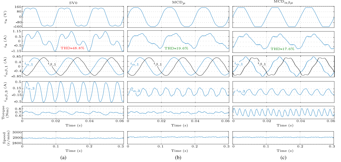
Fig. 8. Experimental results of S6N1 in the time domain of (a) SV0, (b) MCD_\mu , and (c) MCD_{\alpha\beta\mu} for M = 1.10 . From top to bottom: inverter pole-voltage reference of phase a v_a ; current of phase a i_a ; \alpha\beta_1 current; \alpha\beta_3 current; electromagnetic torque; and rotor speed.
