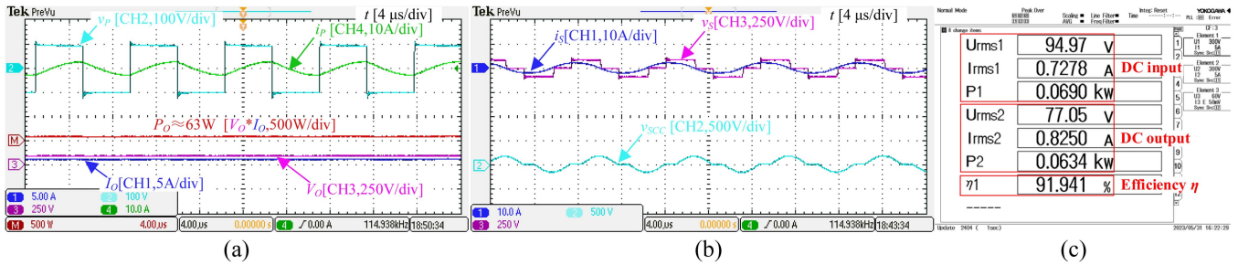
Fig. 15. Captured steady-state waveforms under P_{O,\text{ref}3} = 63\text{ W} . The coupling coefficient is k = 0.3 , R_L = 90\ \Omega . (a) Operating waveforms of the inverter, and the dc output. (b) Operating waveforms of the SCC, and the SAR. (c) Screen capture of DC-to-DC efficiency measurement.
