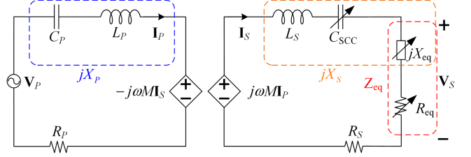
Fig. 5. Equivalent mutual inductance circuit model.
