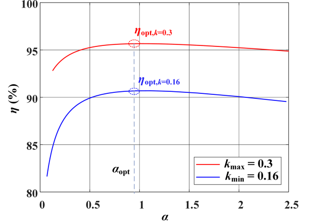
Fig. 6. DC-to-DC efficiency \eta versus current ratio \alpha under different values of k . (Parameters used for simulation are: L_P = 147.23 \mu\text{H} , L_S = 148.5 \mu\text{H} , R_P = 0.451 \Omega , and R_S = 0.52 \Omega . Unless specified, they will be used for the rest simulation.)
