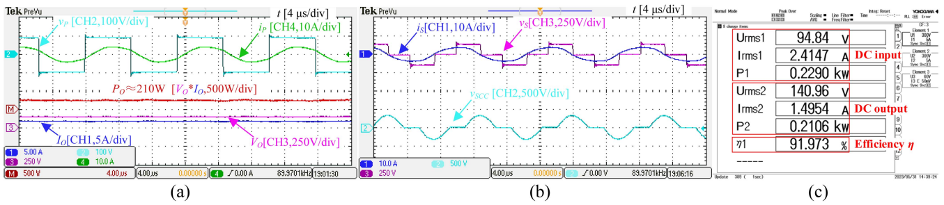
Fig. 14. Captured steady-state waveforms under P_{O,\text{ref}2} = 210\text{ W} . The coupling coefficient is k = 0.3 , R_L = 90\ \Omega . (a) Operating waveforms of the inverter, and the dc output. (b) Operating waveforms of the SCC, and the SAR. (c) Screen capture of DC-to-DC efficiency measurement.
