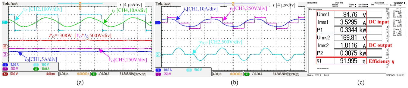
Fig. 13. Captured steady-state waveforms under P_{O,\text{ref}1} = 308\text{ W} . The coupling coefficient is k = 0.3 , R_L = 90\ \Omega . (a) Operating waveforms of the inverter, and the dc output. (b) Operating waveforms of the SCC, and the SAR. (c) Screen capture of DC-to-DC efficiency measurement.
