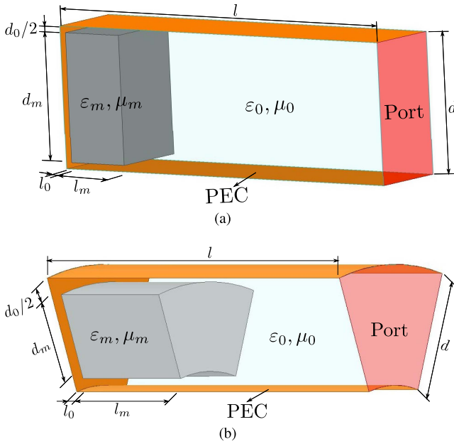
Fig. 4. Geometrical setups used, showing dimensions and boundary conditions used to perform FEM simulations. (a) Cartesian setup. (b) Coaxial setup.
