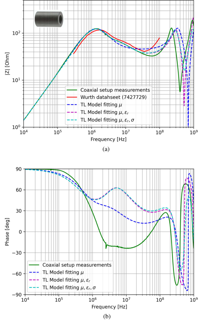
Fig. 7. Plot of experimental measurements of the Wurth 7427729 ferrite in coaxial setup (green) which were the target of the fitting procedure. Results for the fittings permeability parameters with vacuum permittivity (blue), with dielectric permittivity (magenta), and with a conductor (cyan). The manufacturer data (red) is shown for comparison. The observed differences low frequency differences are attributed to differences in the sample ( \pm 25\% tolerance is expected). The differences above 50 MHz are likely to be produced by differences in the experimental setup. (a) Magnitude. (b) Phase.
