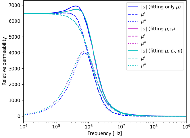
Fig. 8. Permeabilities obtained from the different fittings: Vacuum permeability (blue), with dielectric permittivity (magenta), and with a conductor (cyan). The fittings for dielectric and conductive-type effective permittivities are overlapped.
