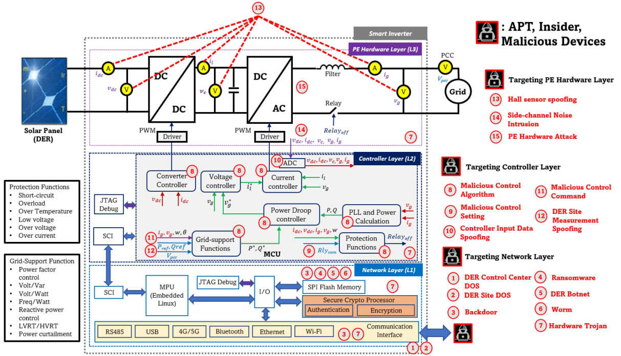
Fig. 2. Practical cyberattack model targeting security-sensitive layers of a smart inverter.
