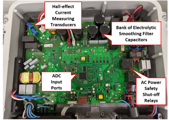
Fig. 4. PE hardware layer attack points.
