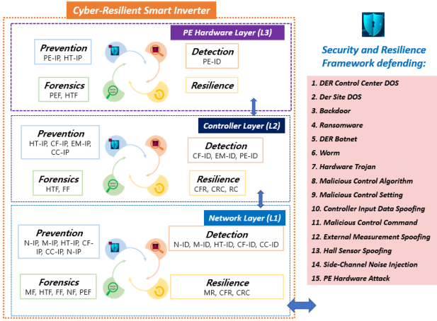
Fig. 5. Cyber-resilient smart inverter security and resilience by design based on the smart inverter security and resilience framework.
