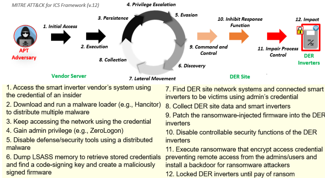
Fig. 3. Ransomware attack model targeting DER smart inverters through an inverter vendor's OTA firmware update system.
