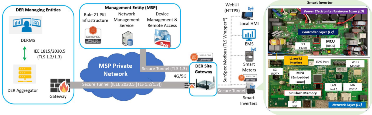
Fig. 1. Practice architecture of the DER system incorporating smart inverters.
