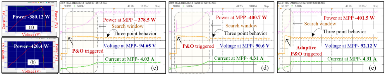
Fig. 14. Programmed P-V characteristics of PV simulator. (a) TCT arrangement. (b) SOPS arrangement. Experimental results for (c) P&O method in TCT arrangement, (d) P&O method in SOPS arrangement, and (e) adaptive P&O in SOPS arrangement—soiling case 2.
