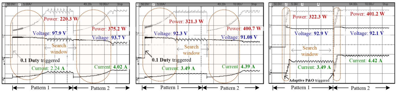
Fig. 17. Experimental results for irradiation change from case 1 to case 2. (a) P&O method in TCT arrangement. (d) P&O method in SOPS arrangement. (e) Adaptive P&O in SOPS arrangement.
