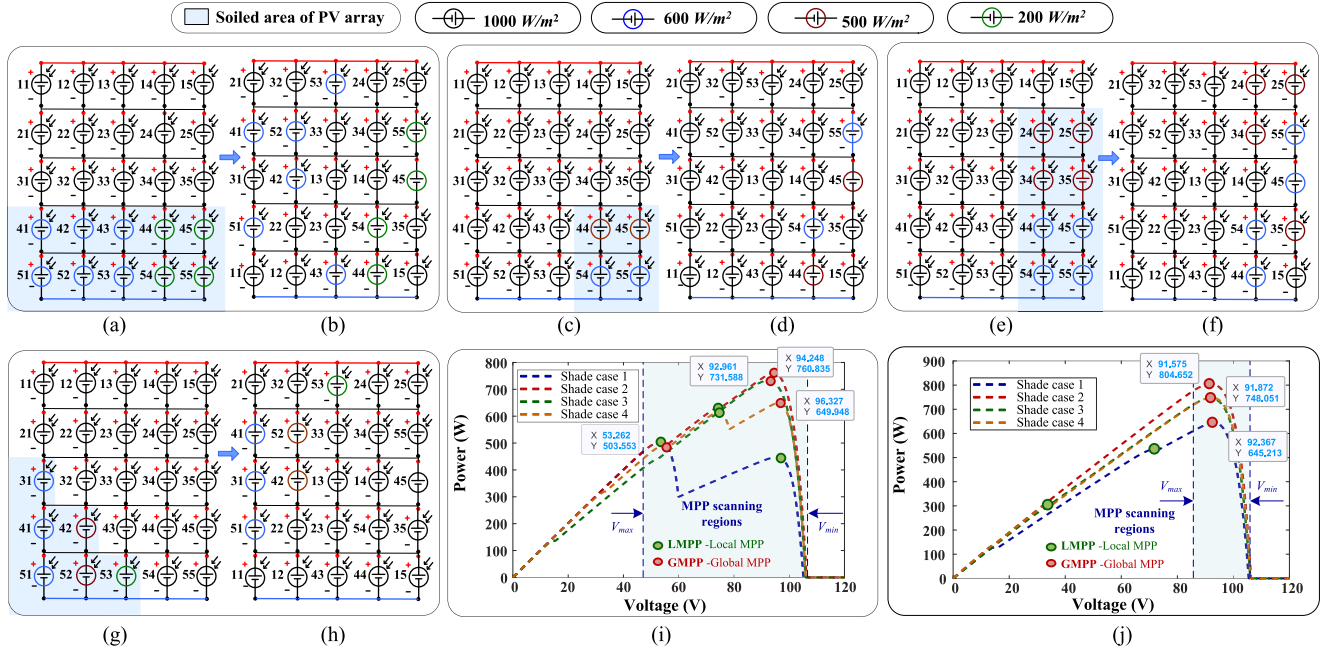
Fig. 9. Soiled case 1: (a) conventional and (b) SOPS PV array; soiled case 2: (c) conventional and (d) SOPS PV array; soiled case 3: (e) conventional and (f) SOPS PV array; soiled case 4: (g) conventional and (h) SOPS PV array; P-V characteristics for Cases 1–4: (i) conventional and (j) SOPS rewired PV array, (note: wiring color– +ve rail – red, –ve rail – blue).
