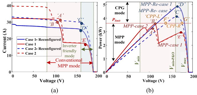
Fig. 4. Illustration of CPG and MPP modes in conventional SP and rewired TCT interconnected PV array. (a) I-V and (b) P-V characteristics.
