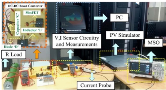
Fig. 12. Laboratory prototype for experimental testing.
