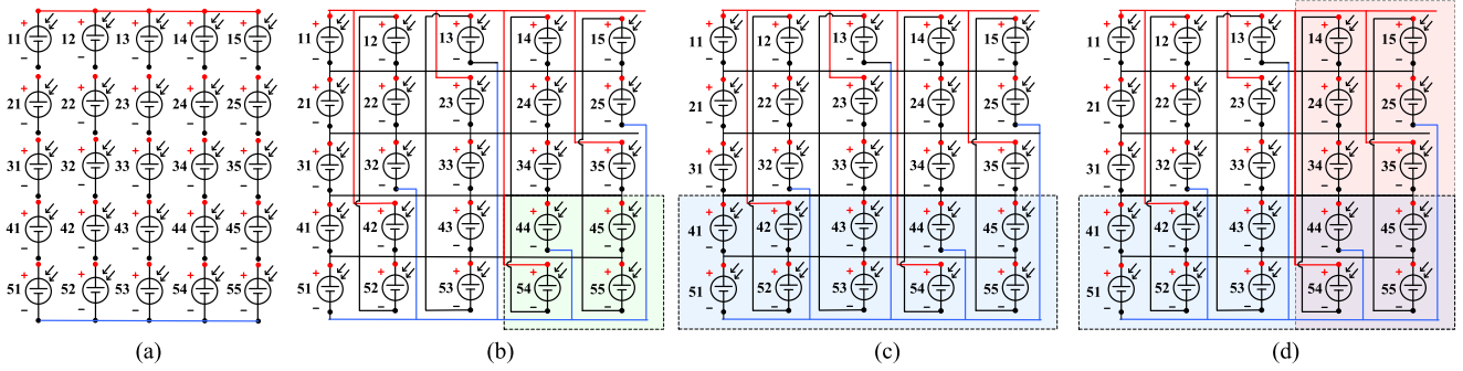
Fig. 2. 5 \times 5 PV arrangement for (a) conventional series–parallel connection, rewired TCT in soiled conditions: (b) low (4 modules shaded), (c) moderate (10 modules shaded), and (d) heavy shading (16 modules shaded), note: Wiring color– +ve rail– red, –ve rail–blue.
