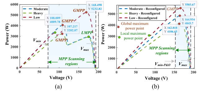
Fig. 3. PV characteristics of (a) conventional and (b) reconfigured PV array.
