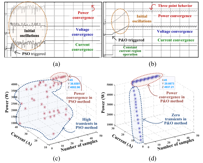
Fig. 5. Experimental results for MPP tracking. (a) PSO method. (b) P&O method; switching transient 3D plot. (c) PSO method. (d) P&O methods.
