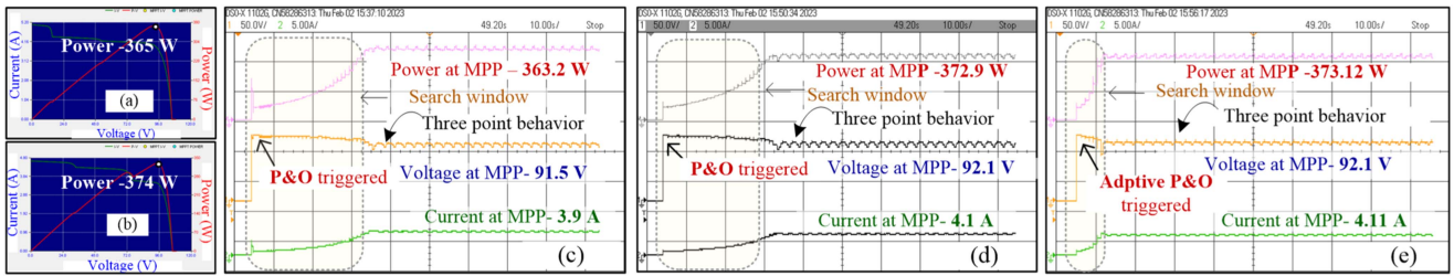
Fig. 15. Programmed P-V characteristics of PV simulator. (a) TCT arrangement. (b) SOPS arrangement. Experimental results for (c) P&O method in TCT arrangement, (d) P&O method in SOPS arrangement, and (e) adaptive P&O in SOPS arrangement—soiling case 3.
