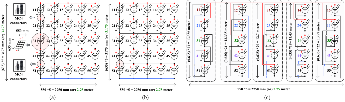
Fig. 10. Wiring length and connector requirements for (a) series parallel (SP), (b) TCT, and (c) SOPS interconnection, (note: wiring color- +ve - red, -ve - blue).
