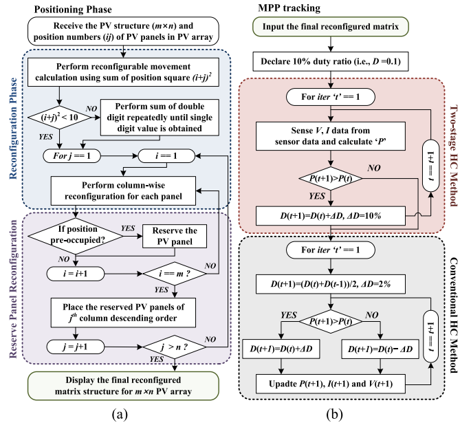
Fig. 8. Generalized flowchart for (a) SOPS Approach and (b) two-phase/adaptive P&O tracking.
