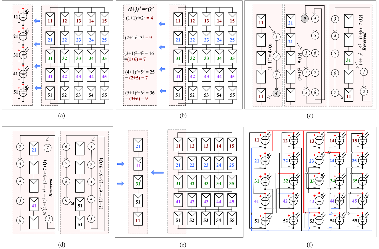
Fig. 6. Illustration of the SOPS method— 5 \times 5 PV array. (a) Simple TCT interconnection. (b) Determining “ Q ” value for the first column based on SOPS procedure. (c) Rewiring the first column elements “11,” “21,” and “31.” (d) Rewiring the first column elements “41” and “51.” (e) Illustration of the “reserved” PV panels in the first column. (f) Final PV arrangement of SOPS-PV arrangement. (Note: wiring color— +ve rail – red, –ve rail – blue).
