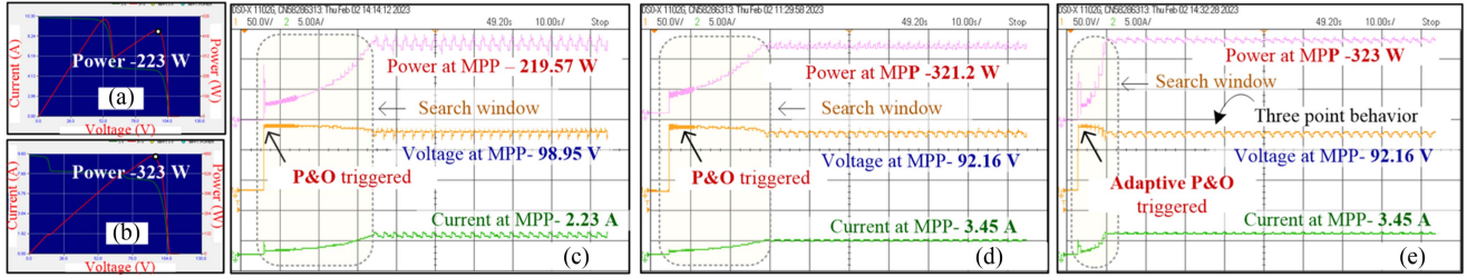
Fig. 13. Programmed P-V characteristics of PV simulator. (a) TCT arrangement. (b) SOPS arrangement. Experimental results for (c) P&O method in TCT arrangement, (d) P&O method in SOPS arrangement, and (e) adaptive P&O in SOPS arrangement—soiling case 1.
