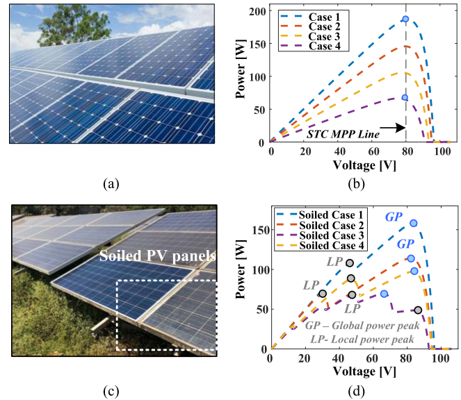
Fig. 1. Normal operating conditions (a) PV array, (b) P-V characteristics, soiled conditions, (c) PV array, and (d) P-V characteristics.
