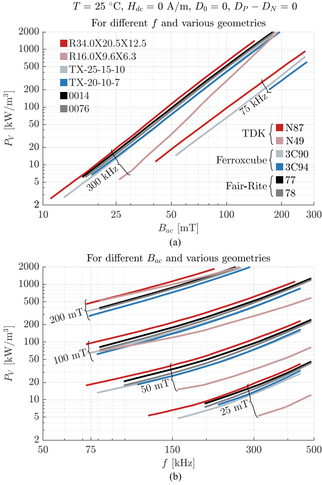
Fig. 31. Core losses for different Mn-Zn materials for a triangular 50% duty cycle excitation without dc bias at 25 °C. (a) As a function of B_{ac} for a set of frequencies. (b) As a function of f for different values of B_{ac} .
