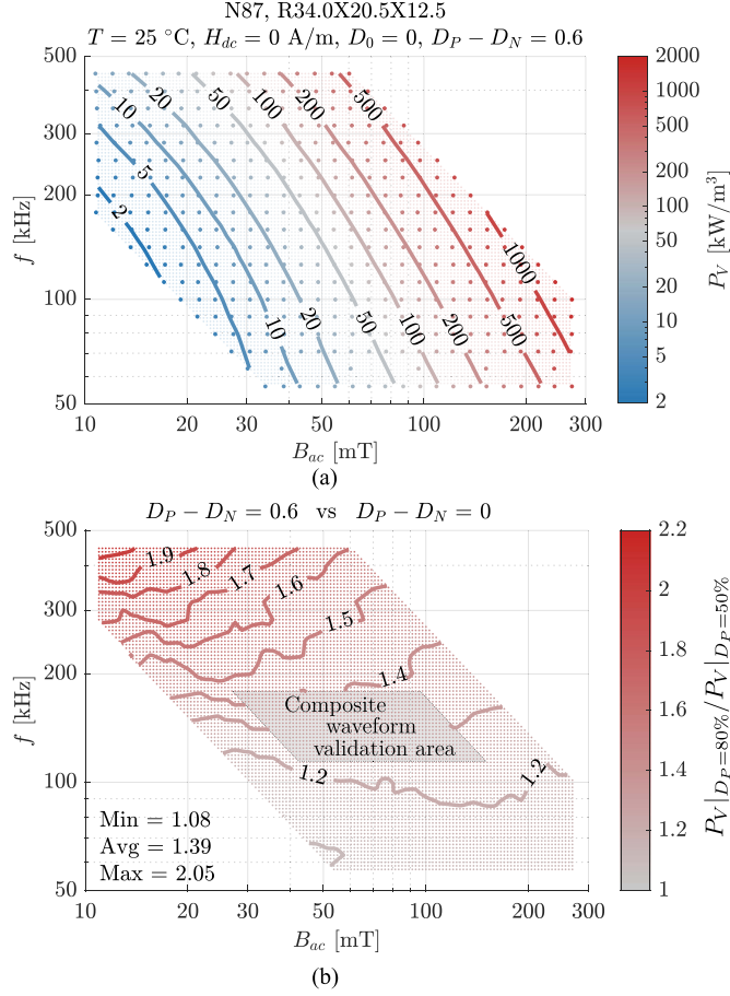
Fig. 17. Effect of duty cycle in volumetric core losses. (a) Core losses for triangular 80% duty cycle excitations without dc bias at 25^\circ\text{C} as a function of B_{ac} and f . (b) Ratio between P_V at 80% duty cycle and 50% duty cycle. The composite waveform hypothesis has been tested in the marked area.
