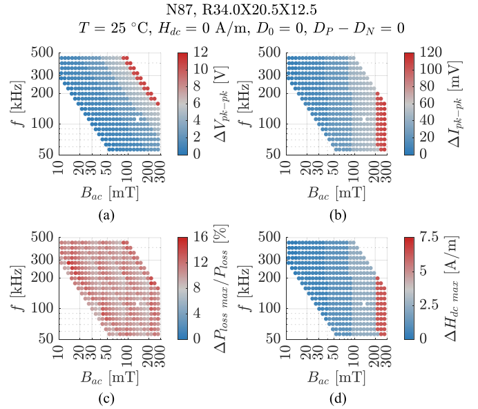
Fig. 40. Effect of the gain and offset errors in the measurements of N87 triangular 50% waveforms at 25 °C without dc bias. (a) Worst case error because of the passive probe and scope in the peak-to-peak voltage measurement. (b) Worst case error because of the passive probe and scope in the peak-to-peak current measurement. (c) Worst case relative error in the core loss; calculated as (V_{pk-pk} + \Delta V_{pk-pk}) \cdot (I_{pk-pk} + \Delta I_{pk-pk}) / (V_{pk-pk} \cdot I_{pk-pk}) - 1 . (d) Worst case absolute error in dc bias due to offset.
