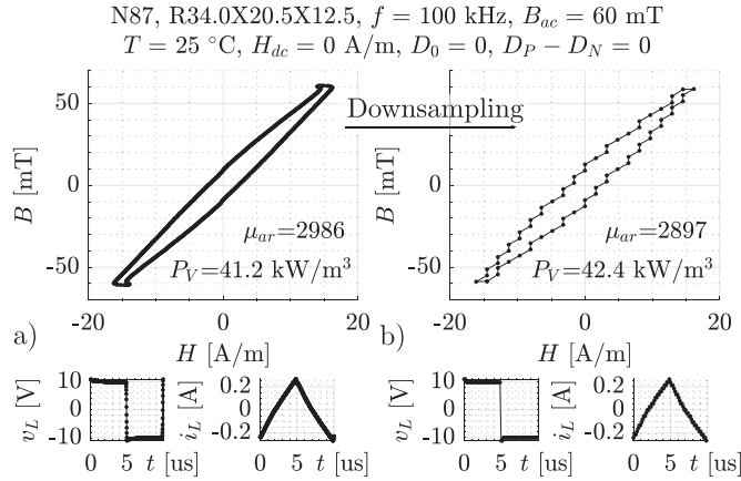
Fig. 41. B - H loops for one of the measured waveforms with the values of amplitude permeability and core loss calculated from the B and H signals. (a) Measured B - H loop. (b) Downsampling the number of points per cycle from 1024 to 64 and rounding V and I to one-tenth of their respective peak-to-peak values. The effect on losses and permeability is not so significant even in such an extreme case.
