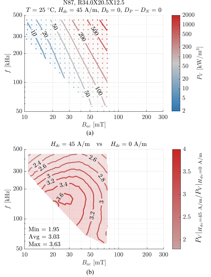
Fig. 23. (a) Core losses for a triangular 50% duty cycle excitation at 25 °C and 45 A/m as a function of B_{ac} and f . (b) Ratio between losses in (a) and without dc bias (see Fig. 11). This ratio is referred to as the displacement factor in [67].
