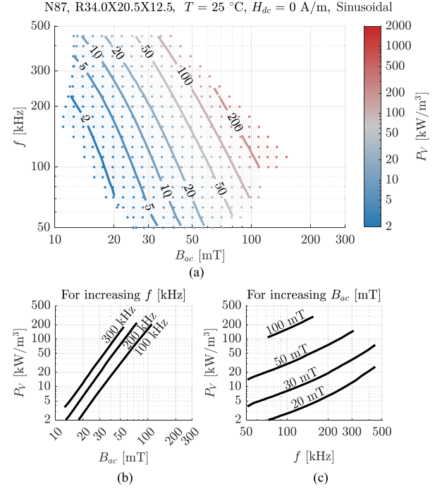
Fig. 7. Volumetric core losses for sinusoidal excitations at 25 °C without dc bias for data with \text{THD}_V < 5\% . (a) As a function of B_{ac} and f (termed f - B_{ac} plane). Each dot is a measured value. The contours are based on the interpolation of the measurements. (b) For various frequencies as a function of B_{ac} . (c) For various B_{ac} as a function of f .
