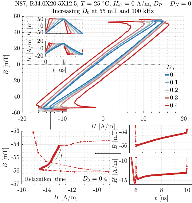
Fig. 19. Measured B - H loops for trapezoidal waveforms of different relaxation time and dB/dt at 25 °C, 100 kHz, and 55 mT without dc bias. A zoom of the negative dB/dt \approx 0 part for D_0 = 0.4 on the region where B and H are nearly constant is also included.
