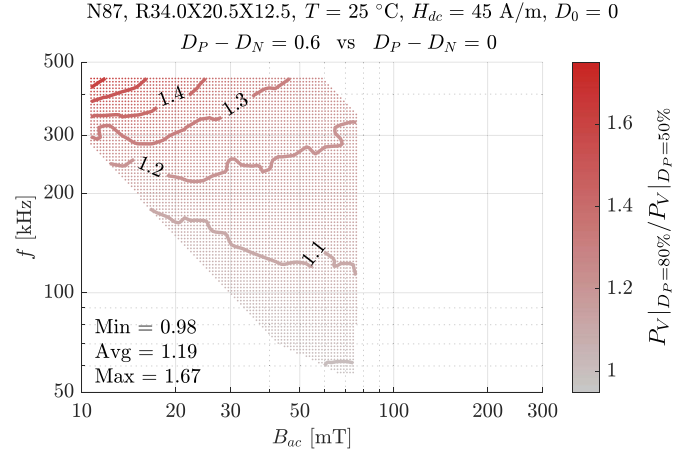
Fig. 36. Ratio between P_V at 80% and 50% duty cycle at 45 A/m. The range is limited to the frequencies and flux densities where data are available for both duty cycles. Compare with the data at 0 A/m in Fig. 17(b).
