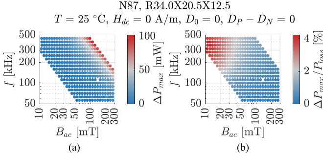
Fig. 38. Effect of 1.6-ns delay between the voltage and current measurement on a subset of the N87 data. (a) Worst case added or subtracted losses. (b) Relative error.
