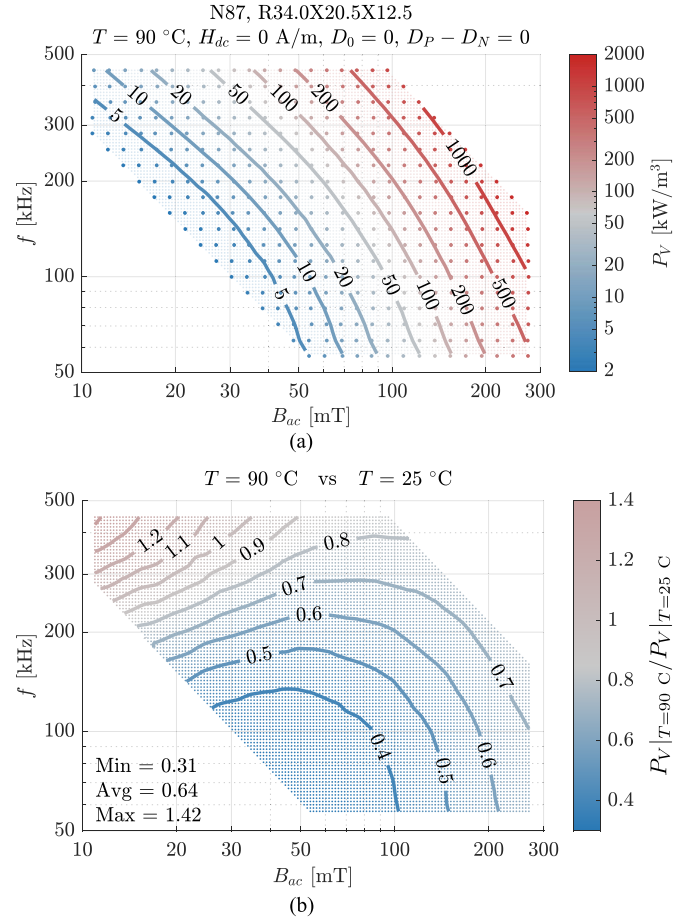
Fig. 26. (a) Core losses for a triangular 50% duty cycle excitation without dc bias at 90 °C as a function of B_{ac} and f , for comparison with the data in Fig. 11 at 25 °C. (b) Ratio between the volumetric core loss at 90 °C and 25 °C.
