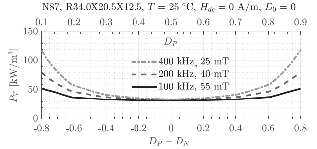
Fig. 16. Effect of duty cycle on core losses for triangular excitations without dc bias at 25^\circ\text{C} at the B_{ac} and f for the waveforms in Fig. 14 and two more B_{ac} and f combinations with similar losses at 50% duty cycle.
