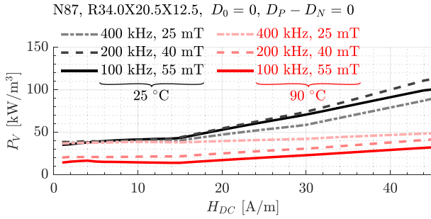
Fig. 35. Core loss against dc bias for triangular 50% duty cycle waveforms at 25 °C and 90 °C. for a few combinations of B_{ac} and f . The same interpolation used in Fig. 22 is selected.
