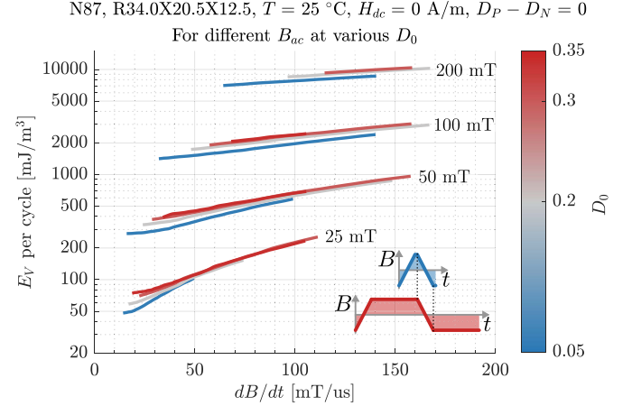
Fig. 20. Energy loss per cycle losses as a function of the duty cycle of the zero-voltage region, D_0 , for trapezoidal symmetric excitation at 25 °C and without dc bias as a function of the dB/dt of the rising and falling parts of the trapezoidal waveform for given flux densities.
