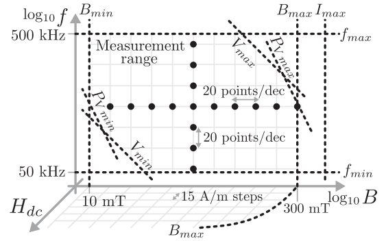
Fig. 4. Range for the tests for the B_{dc} , f , and H_{dc} variables.
