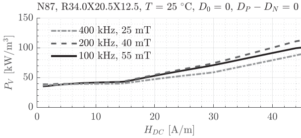
Fig. 22. Interpolated core losses as a function of H_{dc} for a few combinations of B_{ac} and f for 50% duty cycle triangular excitation at 25 °C. Instead of interpolating for H_{dc} directly, \log_{10}|H_{dc}| is used as it provides more reasonable results. Note that data are measured in steps of 15 A/m.
