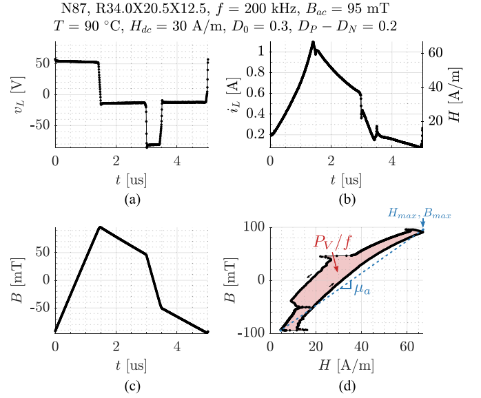
Fig. 5. Processed measurements for a random asymmetric trapezoidal waveform. (a) Measured voltage. (b) Measured current and magnetic field intensity. (c) Flux density. B_{dc} is not included. (d) B - H loop highlighting P_V and \mu_a , as defined in (5).
