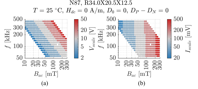
Fig. 39. Scale for the voltage and current used for the tests for triangular 50% duty cycle waveforms at 25 °C without dc bias measurements.
