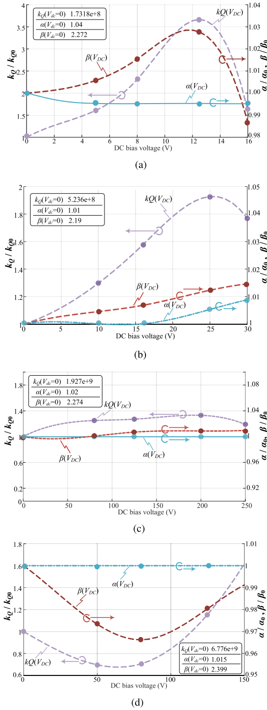
Fig. 11. Changes of the coefficients in SE according to varying dc bias voltage. (a) C3216X5R1E106K160: X5R-LV. (b) C3216X7R1V225K160: X7R-LV. (c) C4532X7T2W474K230: X7T-HV. (d) C5750X7R2E105K230: X7R-HV.
