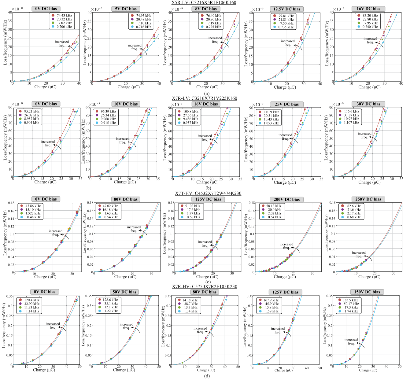
Fig. 10. Measured power loss/frequency ( P/f ), which physically represents energy enclosed per Q - V loop, against measured charge Q_{pk} of four CUTs. (a) C3216X5R1E106K160 using LV X5R dielectric. (b) C3216X7R1V225K160AE using LV X7R dielectric. (c) C4532X7T2W474K230KE using HV X7T material. (d) C5750X7R2E105K230KE using HV X7R material. In the test, both the frequency and the applied charge Q_{pk} were varied and different loss dependencies on frequency and DC-bias-voltage can be observed on these four types of dielectric materials.
