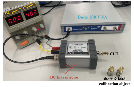
Fig. 19. Small-signal capacitance measurement with the presence of DC bias voltage using one-port ( S_{11} ) measurement. Short, load, and open calibration objects are needed to ensure accuracy.
