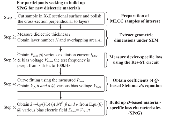
Fig. 14. Process for establishing the loss characteristic of new ferroelectric dielectric material.
