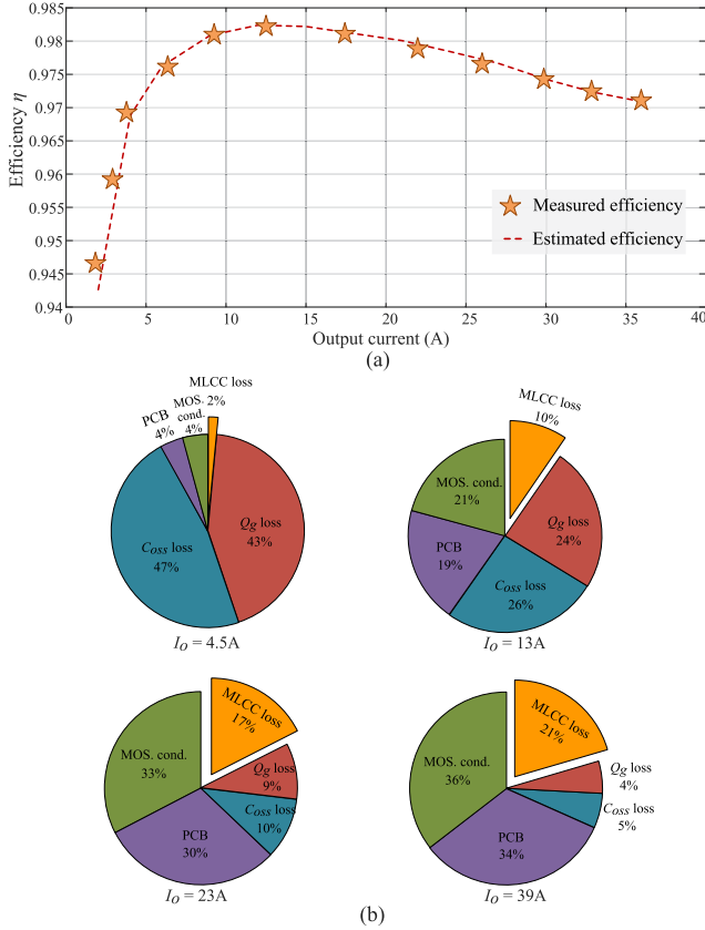
Fig. 26. (a) Comparison between measured and estimated efficiency curves. (b) Loss breakdown of the prototype at four different load conditions.
