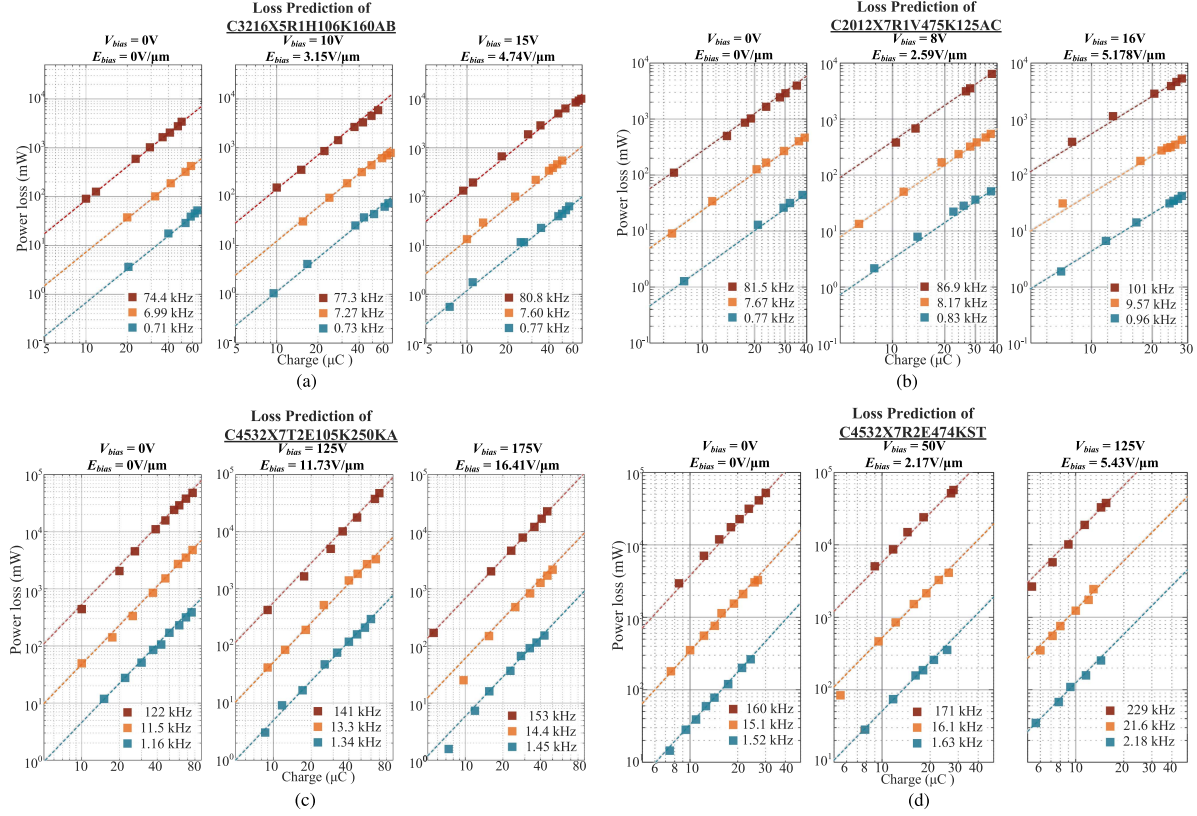
Fig. 22. Logarithmic representation of measured power loss against peak-peak charge Q_{pk} with an increased DC bias voltage of four MLCC samples using different dielectric materials: (a) C3216X5R1H106K160AB, (b) C2012X7R1V475K125AC, (c) C4532X7T2E105K250KA, and (d) C4532X7R2E474KST. Squares represent the measurement results and dotted lines denote the calculated power losses using the material-specific SE coefficients obtained from the SPeGs given in Fig. 20.
