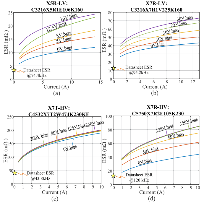
Fig. 12. ESR characteristics of four Class II MLCC samples at high frequency across various DC bias voltages: (a) C3216X5R1E106K160 (@ 74.4 kHz), (b) C3216X7R1V225K160 (@ 95.2 kHz), (c) C4532X7T2W474K230KE (@ 43.8 kHz), and (d) C5750X7R2E105K230 (@ 120 kHz).
