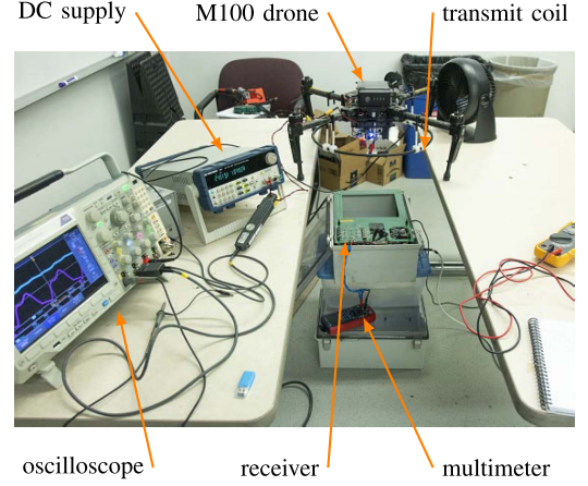
Fig. 20. Test setup in the laboratory.
