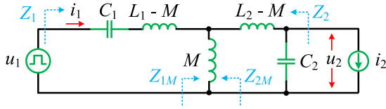
Fig. 4. Simplified model of the S-P compensated IPT system.
