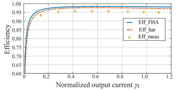
Fig. 18. System efficiency variation when k = 0.8 .
