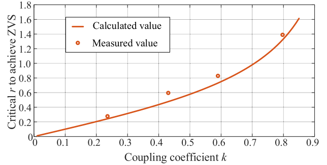
Fig. 14. Critical load current variation versus the coupling coefficient.
