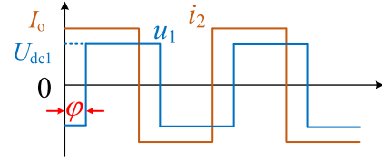
Fig. 3. Theoretical waveforms of the input voltage u_1 and output current i_2 .
