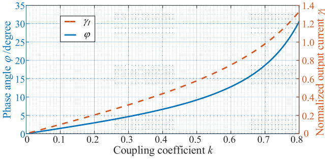
Fig. 8. Phase angle \varphi and \gamma_I to achieve ZVS with different coupling coefficients k .
