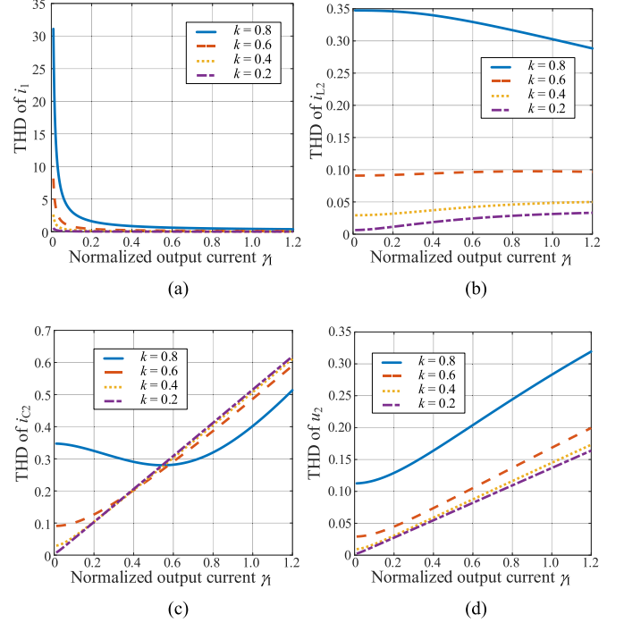
Fig. 9. THDs of i_1 , i_{L2} , i_{C2} , and u_2 . (a) THD of i_1 . (b) THD of i_{L2} . (c) THD of i_{C2} . (d) THD of u_2 .
