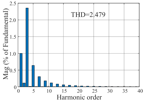
Fig. 16. Harmonic distribution of i_{C1} when k = 0.8 and \gamma_1 = 0.12 .
