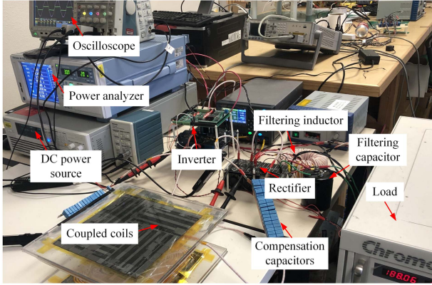
Fig. 12. Experimental platform of an S-P compensated IPT system.
