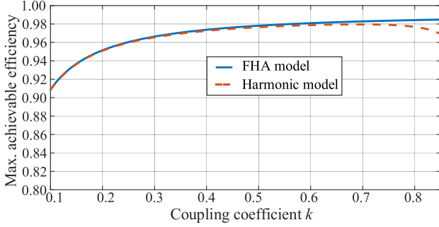
Fig. 10. Variation of the maximum achievable coil-to-coil efficiency.
