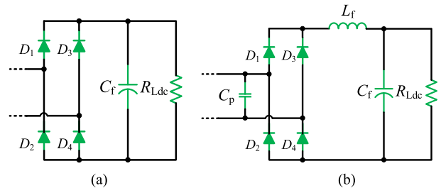
Fig. 1. Two different filters used for the IPT system. (a) Capacitive filter. (b) Inductive filter.
