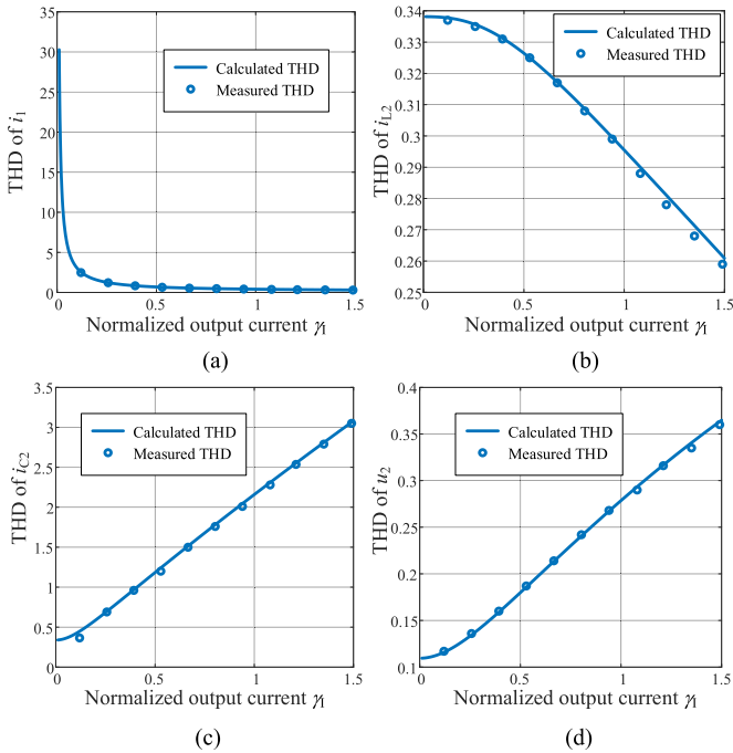
Fig. 15. Calculated and measured THD when k = 0.8 . (a) THD of i_1 . (b) THD of i_{L2} . (c) THD of i_{C2} . (d) THD of u_2 .
