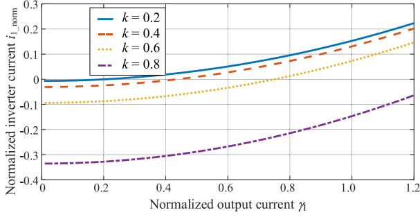
Fig. 7. Normalized i_1(\varphi/\omega_0) with the increasing \gamma_I ( \lambda = 0.5 ).
