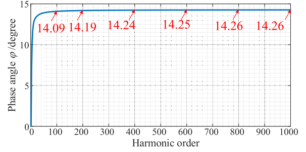
Fig. 5. Variation of \varphi with the increasing harmonic order ( k = 0.8 and \gamma_I = 0.5 ).
