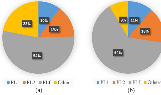
Fig. 20. Power loss distribution when the input power is 409 W and k is 0.8. (a) Calculated power loss distribution. (b) Measured power loss distribution.
