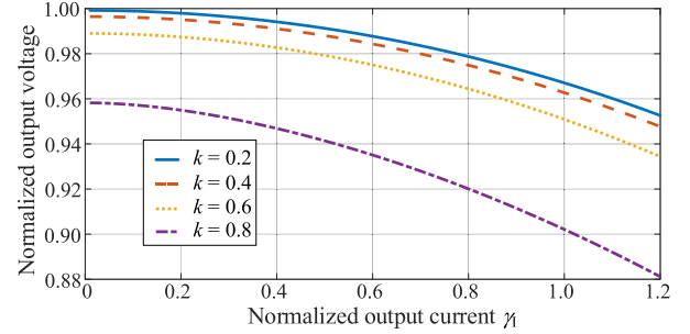
Fig. 11. Output DC voltage characteristics.
