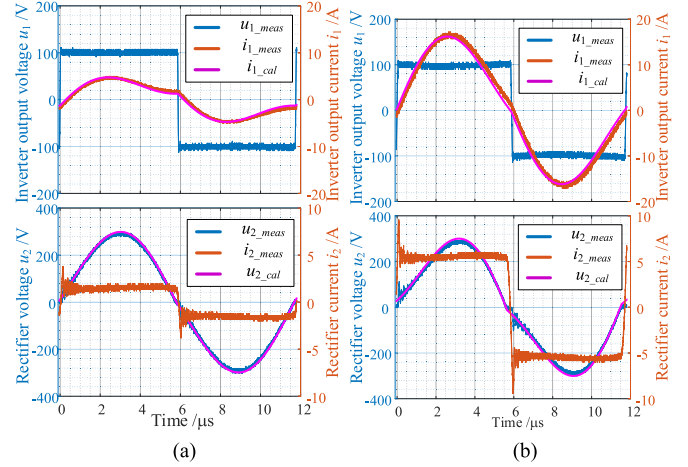
Fig. 13. Experimental waveforms ( k = 0.43 , \lambda = 2.32 ). (a) \gamma_I = 0.174 . (b) \gamma_I = 0.61 .
