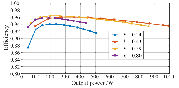
Fig. 17. System efficiency variations with different coupling coefficients.
