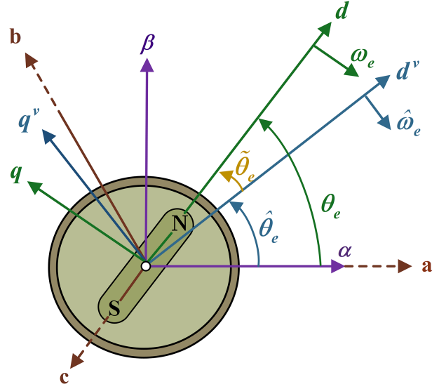
Fig. 2. Different reference frames in a PMSM drive.
