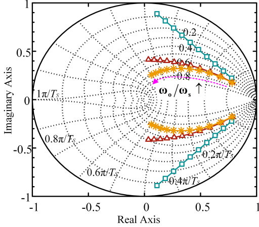
Fig. 11. Discrete-time pole migration comparison with \omega_0 increase [93]. (□: Euler approximation; △: Tustin approximation; *: Exact discretization).
