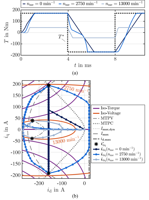
Fig. 7. Simulative TO-MPC trajectories for maximum and minimum torque operation for different speeds n_{\text{me}} with an initial rotor angle \varepsilon(t=0\text{ s})=0 . (a) Torque trajectories. (b) Current trajectories.
