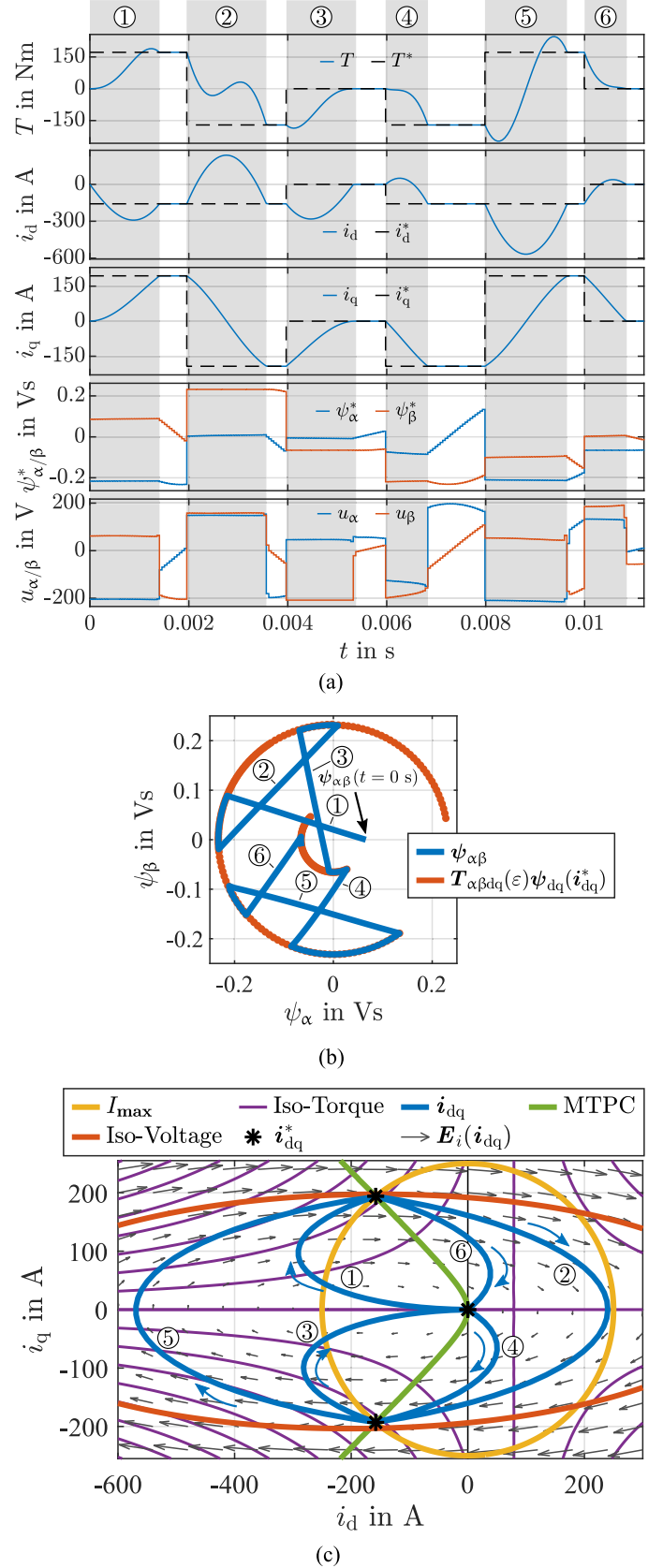
Fig. 3. Exemplary trajectories with the RPR ( t_{\text{thresh}} = 1.5T_s , N = 10 ), the deadbeat flux control law (21), and the initial condition \varepsilon(t = 0\text{ s}) = 0 at nominal speed ( n_{\text{me}} = 2750 \text{ min}^{-1} ). (a) Time courses. (b) Flux linkage trajectories. (c) Current trajectories.
