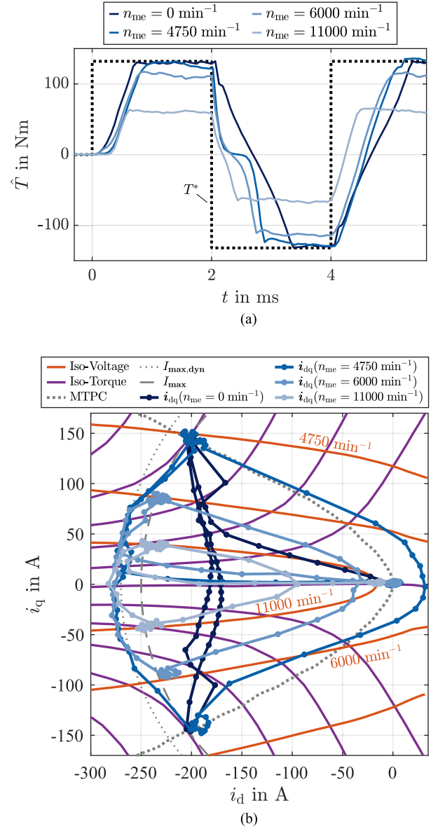
Fig. 13. Experimental TO-MPC trajectories for maximum and minimum torque operation for different speeds n_{me} with an initial rotor angle \varepsilon(t=0\text{ s}) = 0 . (a) Torque trajectories. (b) Current trajectories.
