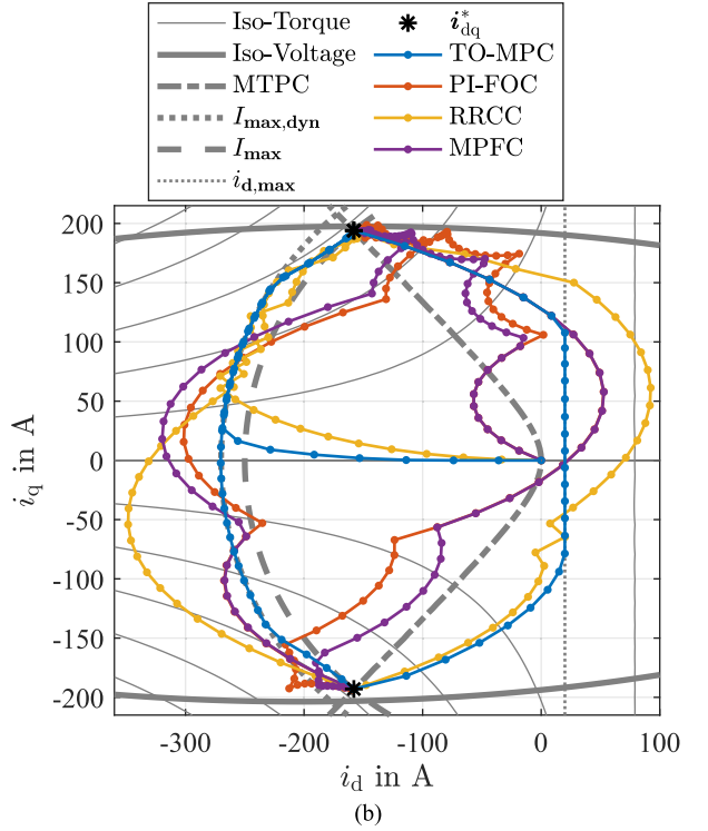
Fig. 8. Simulative trajectories at rated speed ( n_{me} = 2750 \text{ min}^{-1} ) with an initial rotor angle \varepsilon(t = 0\text{ s}) = 0 . (a) Torque trajectories. (b) Current trajectories.
