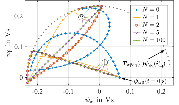
Fig. 4. Flux linkage trajectories for the transients ① and ② of the scenario shown in Fig. 3 for N = \{0; 1; 2; 5; 100\} .
