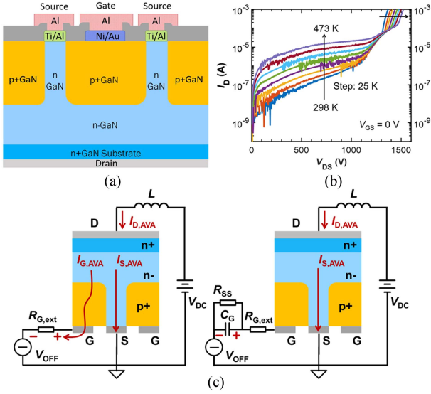
Fig. 14. (a) Schematic of vertical GaN Fin-JFET. (b) Temperature-dependent OFF-state I_D - V_{DS} characteristics. (c) Illustration of the distinct avalanche paths under a MOSFET gate driver and an RC-interface gate driver. Figures adapted from the articles presented in [250] and [252].
