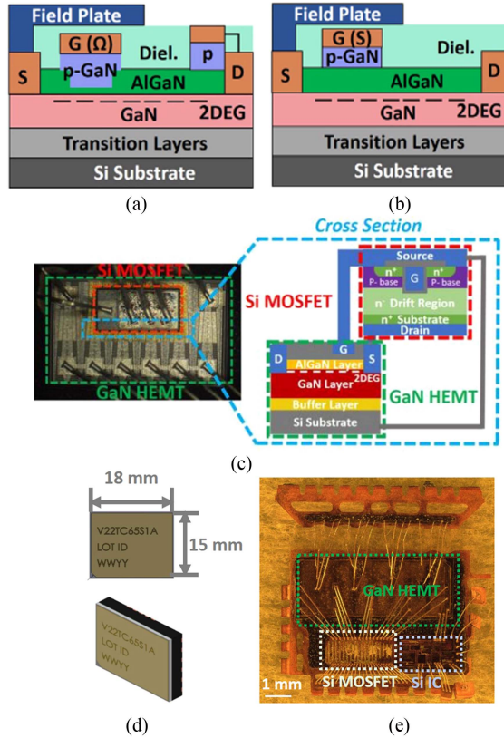
Fig. 2. Schematic of (a) GaN SP-HEMT and (b) GaN HD-GIT. (c) Photograph and schematic of a packaged direct-drive cascode GaN HEMT. (d) Photograph of a packaged direct-drive GaN HEMT. (e) Photograph of a decapsulated direct-drive GaN HEMT from another vendor.
