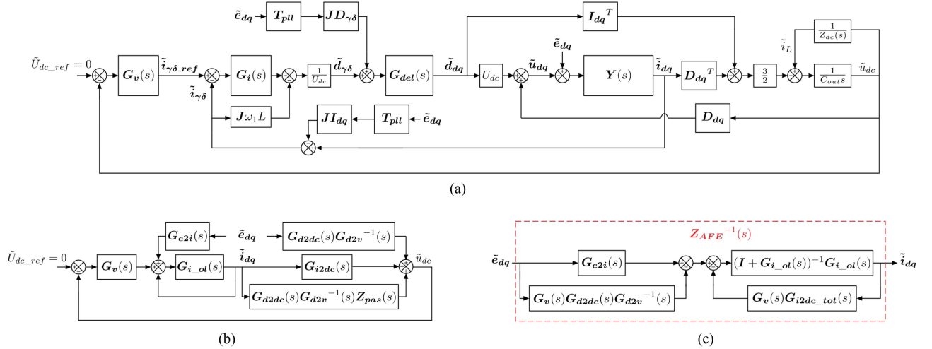
Fig. 3. (a) Small-signal model of the system. (b) Equivalent transformation I. (c) Equivalent transformation II.
