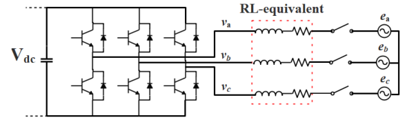
Fig. 1. Topology of a grid-connected voltage source converter.
