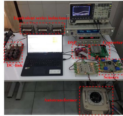
Fig. 12. Picture of the experimental setup.
