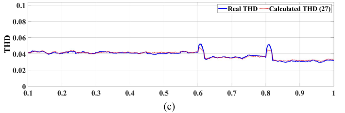
Fig. 9. (a) and (b) Effects of the K factor variation on the current THD. (c) Validation of calculated THD by (27) with real THD.
