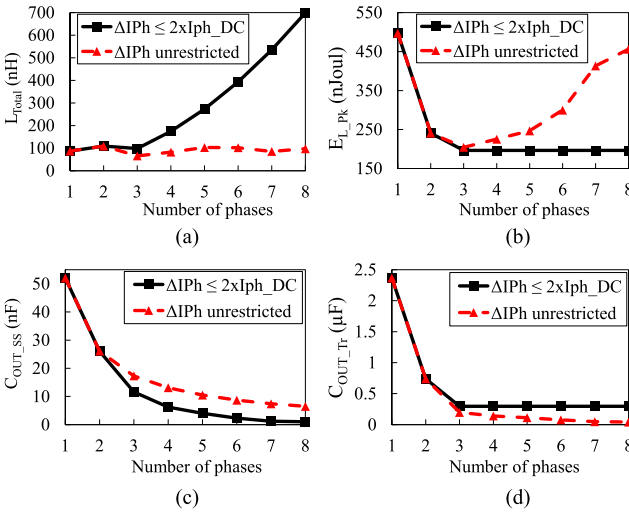
Fig. 7. Passives' analysis versus N_{ph} for converter specification listed in Table I at \Delta I_{ph} < 2\times and 100\times 2I_{ph\_DC} , 100\times limit is considered the unrestricted \Delta I_{ph} case: (a) L_{Tot} , (b) E_{L\_PK} , (c) C_{Out\_SS} , and (d) C_{Out\_Tr} .
