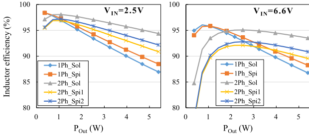
Fig. 10. Calculated inductor efficiency based on measured R_{DC} and R_{AC} .
