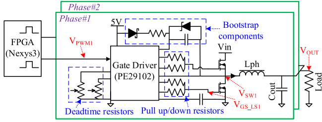
Fig. 12. Circuit schematic of the prototype converter.
