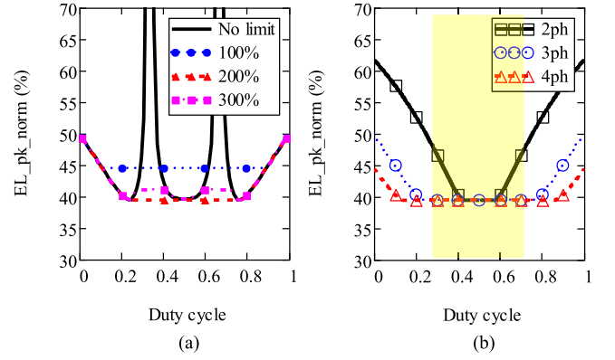
Fig. 3. Inductor analysis at \Delta I_{Nph} = 25\% . (a) Three-phase E_{L\_PK\_norm} at different restriction conditions on \Delta I_{Ph} showing 200% limit energy at minimum for the broadest duty cycle range. (b) E_{L\_PK\_norm} with \Delta I_{Ph\%} restricted at 200%.
