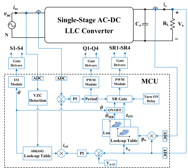
Fig. 13. Digital implementation of the proposed SR driving strategy for the single-stage AC-DC LLC converter.
