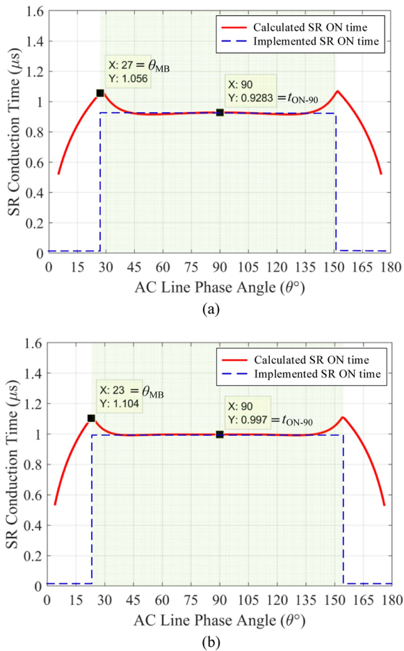
Fig. 10. Calculated SR conduction time at different line phase angles over the AC line half cycle, (a) for V_o = 400 V, P_o = 500 W, and (b) for V_o = 250 V, P_o = 330 W.
