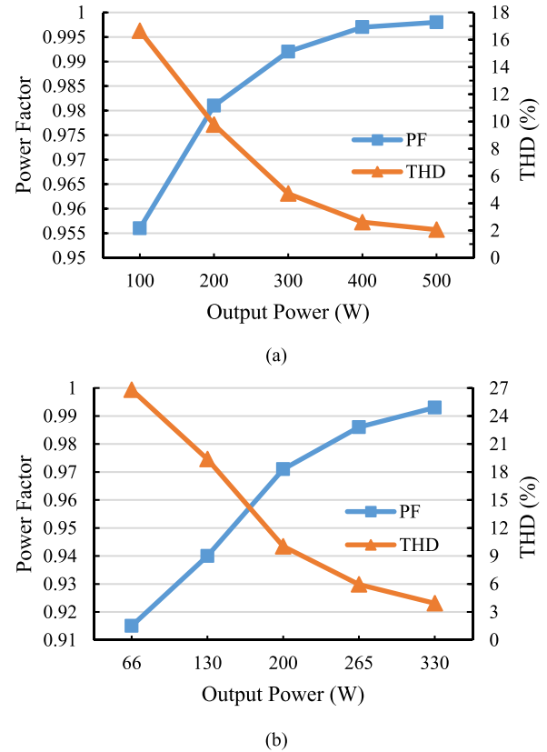
Fig. 16. Measured power factor and THD over the load range for (a) V_o = 400 V, and (b) V_o = 250 V.
