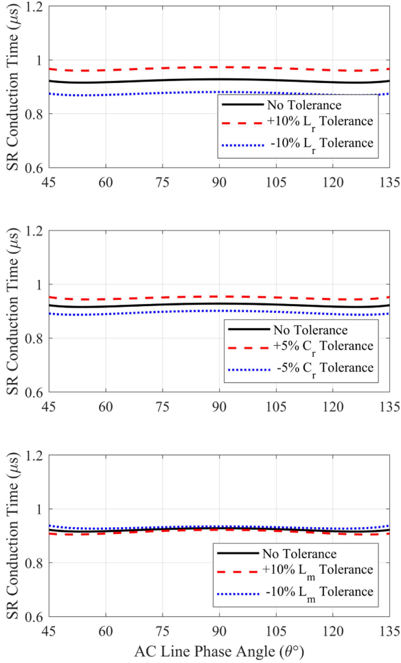
Fig. 11. Calculated SR conduction time considering resonant tank component tolerances for V_o = 400 V.
