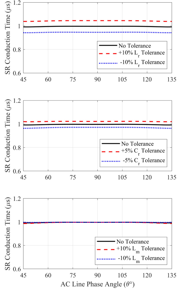
Fig. 12. Calculated SR conduction time considering resonant tank component tolerances for V_o = 250 V.
