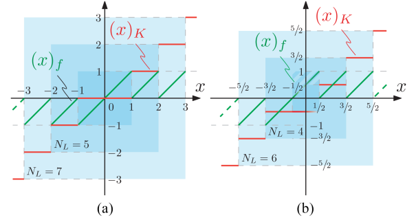
Fig. 3. Graphs of the functions (\cdot)_K and (\cdot)_f for different values of N_L . (a) N_L odd. (b) N_L even. Domain and codomain of the functions depending on the number of levels N_L are highlighted, the inner areas are related to N_L equal to 3 and 2.
