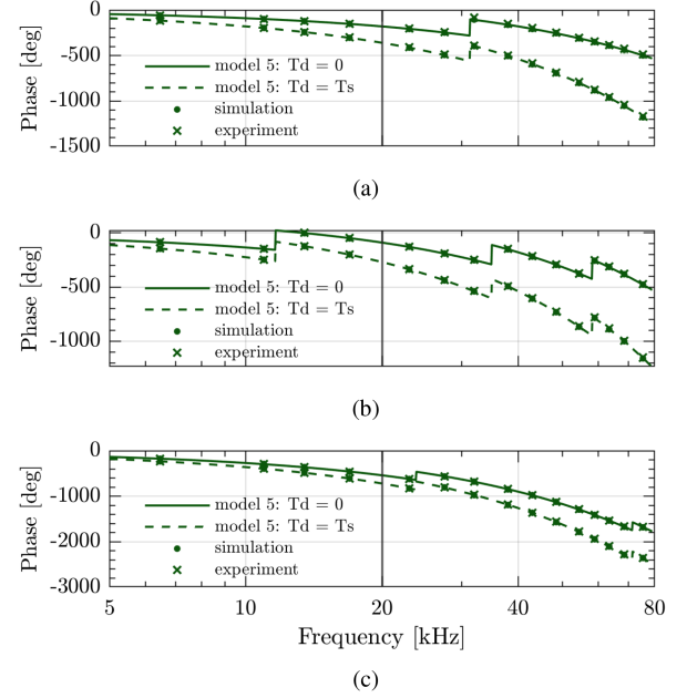
Fig. 10. Phase of the DPWM's frequency response, with T_d = T_s and T_d = 0 , obtained from the proposed model, and simulated and experimental FRMs. (a) U-MSDU-DPWM at M = 0.66 . (b) BPS-MSDU-DPWM at M = 0.79 . (c) UPS-MSDU-DPWM at M = 0.57 . The gray vertical line marks the NF.
