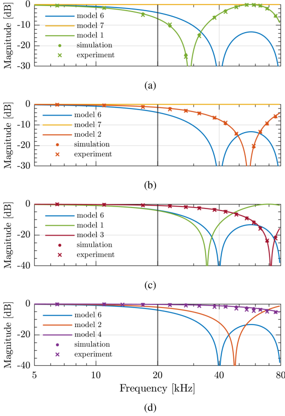
Fig. 7. Magnitude of the DPWM's frequency response obtained from different small-signal models, and simulated and experimental FRMs. (a) DSDU-B-DPWM at M = 0.85 . (b) MSMU-U-DPWM at M = 0.66 . (c) MSMU-BPS-DPWM at M = 0.79 . (d) MSMU-UPS-DPWM at M = 0.57 . The gray vertical line marks the NF.
