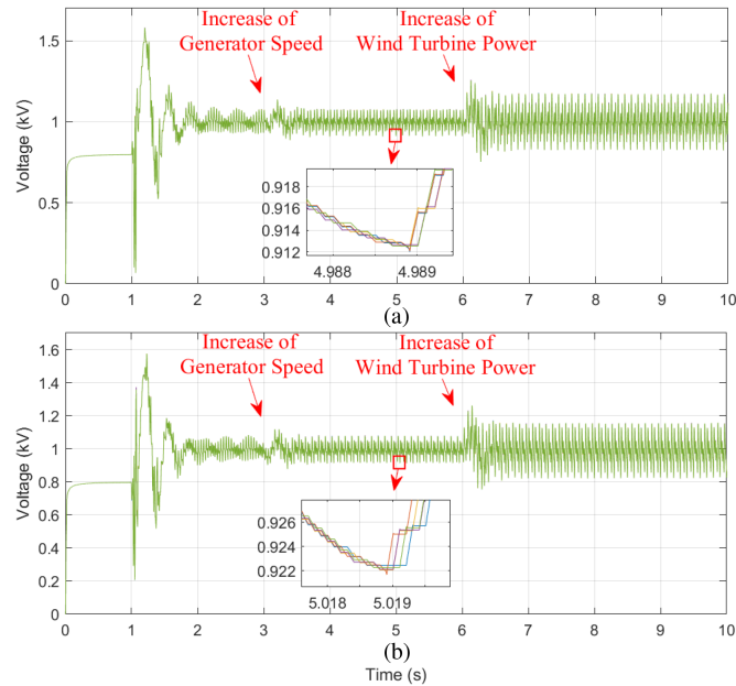
Fig. 16. Simulation results. (a) MMShC phase-A String-X submodule-capacitor voltages. (b) MMShC phase-A String-Y submodule-capacitor voltages.
