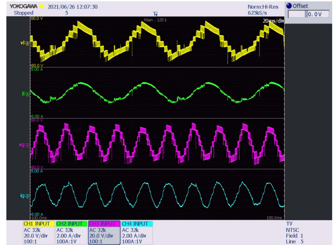
Fig. 18. Experimental results. The first figure (upper one) shown the load-side voltage, the second figure shows the load-side current, the third figure shows the grid-side voltage, and the fourth figure shows the grid-side current.
