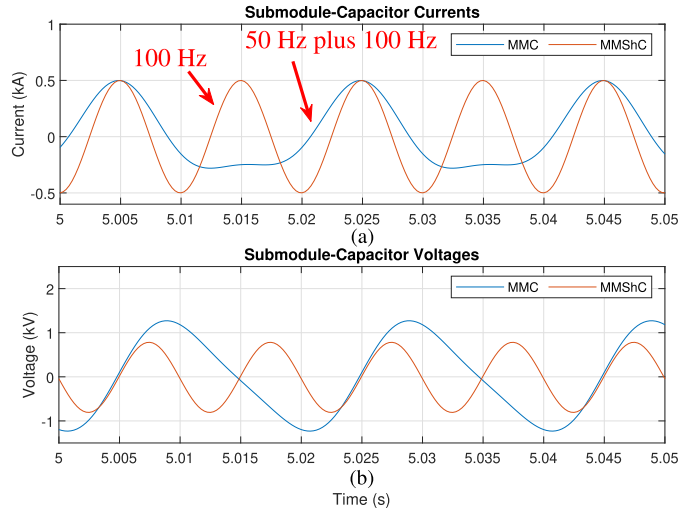
Fig. 10. Simulation results to compare MMC and MMSHC sub-module-capacitor voltage ripple. (a) MMC and MMSHC capacitor currents. (b) MMC and MMSHC sub-module-capacitor voltage ripple.
