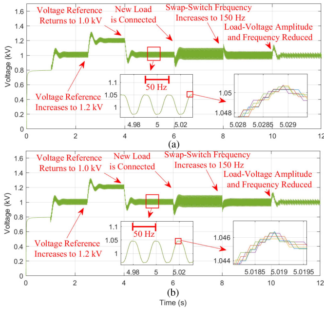
Fig. 14. Simulation results. (a) MMShC phase-A String-X submodule-capacitor voltages. (b) MMShC phase-A String-Y submodule-capacitor voltages.
