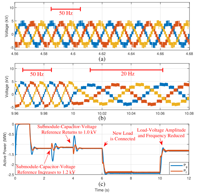
Fig. 12. Simulation results. (a) Voltages synthesized at grid terminals. (b) Voltages synthesized at load terminals. (c) Grid-side and load-side power.
