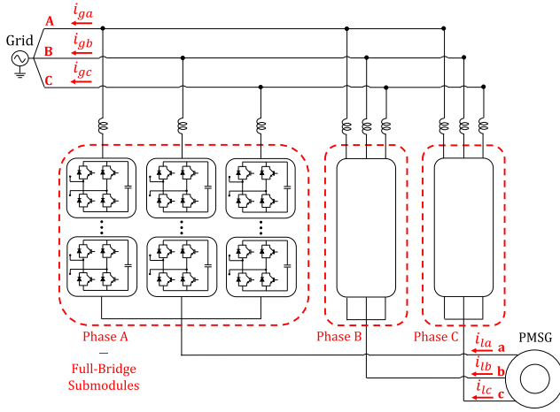
Fig. 7. M 3 C topology.
