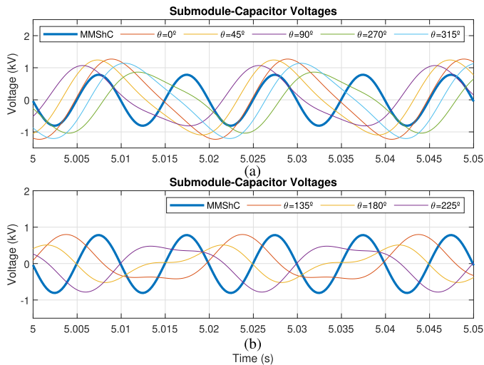
Fig. 11. Simulation results to compare MMC and MMSHC submodule-capacitor voltage ripple. (a) Cases where MMC's submodule-capacitor voltage ripple is higher than MMSHC's one. (b) Cases where MMC's submodule-capacitor voltage ripple is lower than MMSHC's one.
