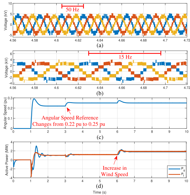
Fig. 15. Simulation results. (a) Voltages synthesized by the MMShC at the grid terminals. (b) Voltages synthesized by the MMShC at the generator terminals. (c) Machine angular speed. (d) Grid-side and generator-side power.
