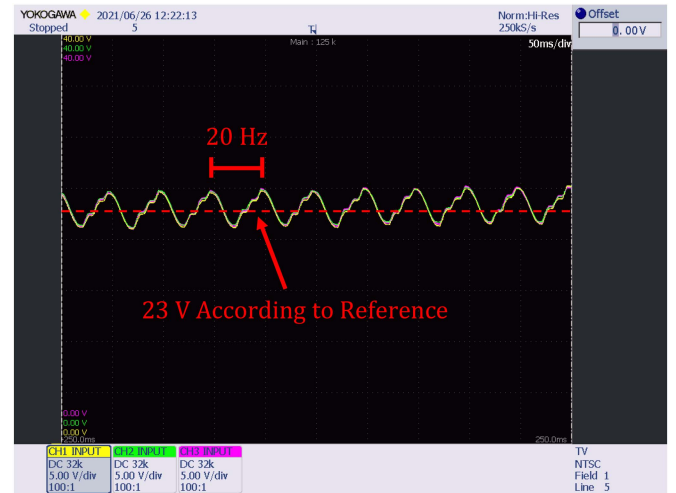
Fig. 19. Experimental results. String-X submodule-capacitor voltages.
