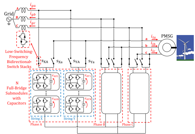
Fig. 1. MMShC topology.
