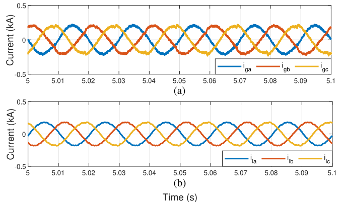
Fig. 13. Simulation results. (a) Grid-side currents. (b) Load-side currents.
