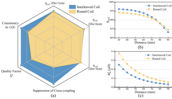
Fig. 12. Comparisons between round coil and interleaved coil designs in a three Tx-UMs three Rx-UMs WPT system. (a) Radar chart. (b) Coil efficiency \eta_{\text{coil}} . (c) Transfer coupling M_{\text{tr}} .
