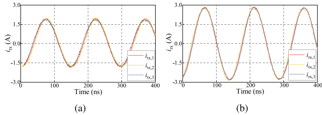
Fig. 18. Current waveforms of UM coils in three Tx-UMs and three Rx-UMs combination. (a) I_{tx,i} . (b) I_{rx,j} .
