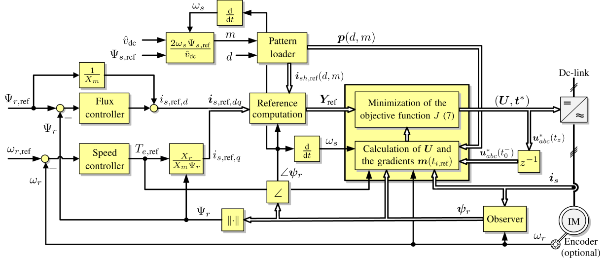
Fig. 2. Block diagram of the GP 3 C scheme.
