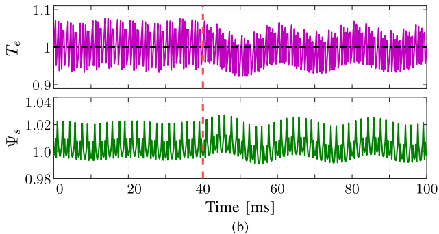
Fig. 18. Response of the system for a change in pulse number from d = 5 to d = 6 while the controller is inactive. (a) Three-phase switching pattern. (b) Torque and stator flux magnitude.
