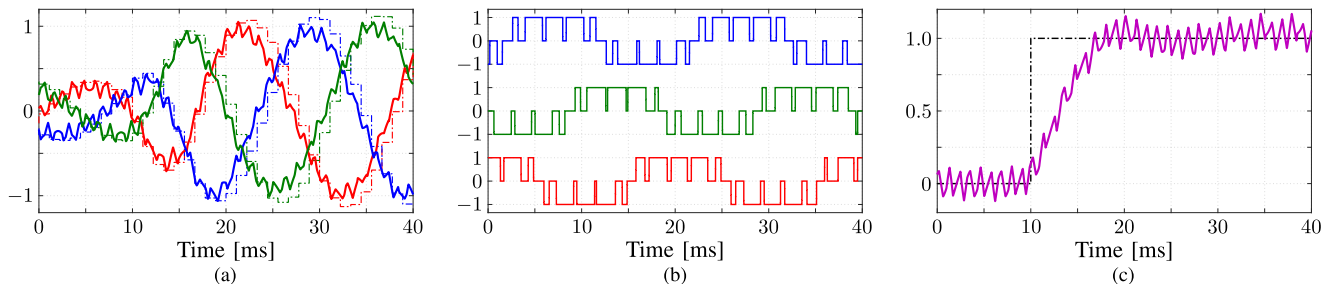
Fig. 13. HIL results produced by FOC during a torque reference step-up change. (a) Three-phase stator current i_{s,abc} (solid lines) and their references (dash-dotted lines). (b) Three-phase switching pattern u_{abc} . (c) Electromagnetic torque T_e (solid line) and its reference (dash-dotted line).
