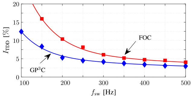
Fig. 8. Tradeoff between stator current TDD I_{TDD} and switching frequency f_{sw} for the proposed GP 3 C (blue) and FOC (red). The individual HIL results are shown as rhombi (GP 3 C) and squares (FOC).
