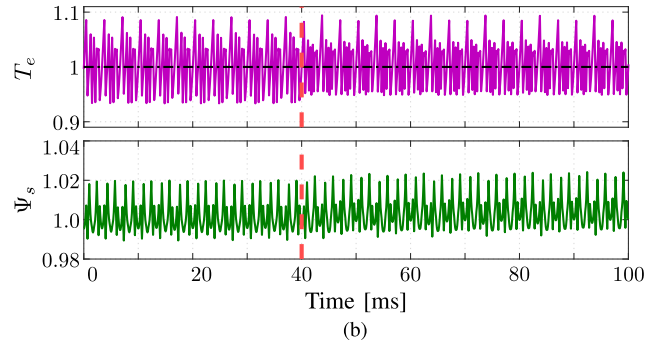
Fig. 19. Response of the system for a change in pulse number from d = 5 to d = 6 when GP 3 C is activated. (a) Three-phase switching pattern. (b) Torque and stator flux magnitude.
