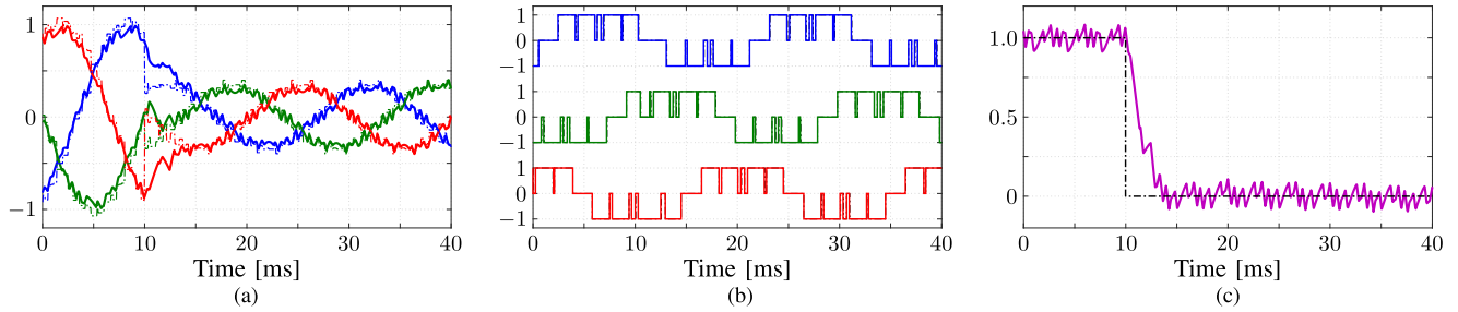
Fig. 10. HIL results produced by the proposed GP 3 C algorithm during a torque reference step-down change. (a) Three-phase stator current i_{s,abc} (solid lines) and their references (dash-dotted lines). (b) Three-phase switching pattern u_{abc} (solid lines) and the nominal OPP (dash-dotted lines). (c) Electromagnetic torque T_e (solid line) and its reference (dash-dotted line).
