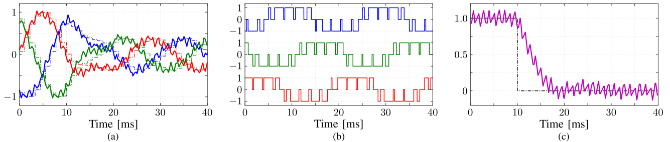
Fig. 12. HIL results produced by FOC during a torque reference step-down change. (a) Three-phase stator current i_{s,abc} (solid lines) and their references (dash-dotted lines). (b) Three-phase switching pattern u_{abc} . (c) Electromagnetic torque T_e (solid line) and its reference (dash-dotted line).
