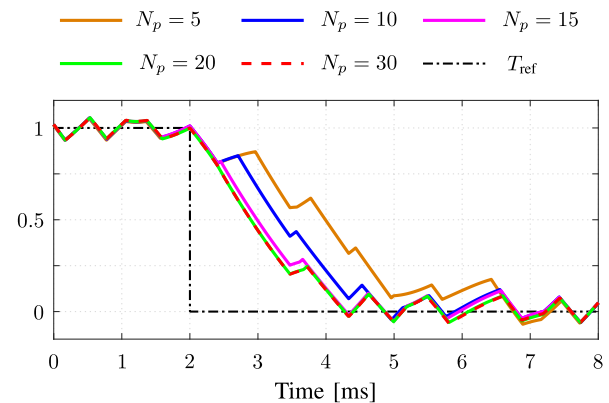
Fig. 20. Torque step-down response when the prediction horizon is varied from N_p = 5 to N_p = 30 .
