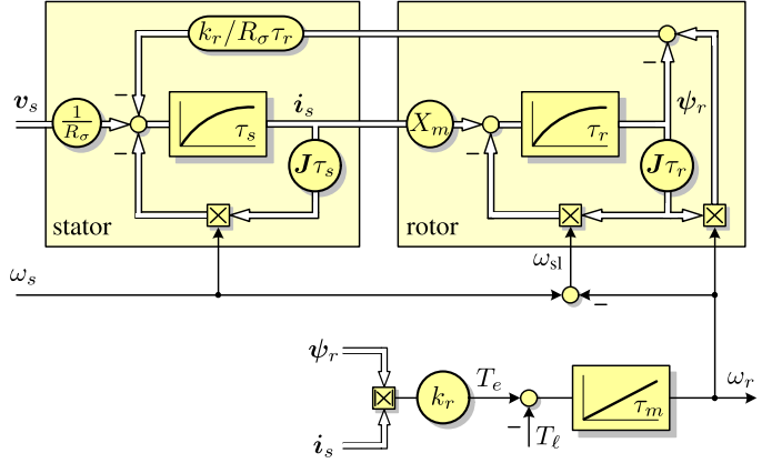
Fig. 5. Signal flow graph of the dynamic induction machine model for real-time HIL system implementation.
