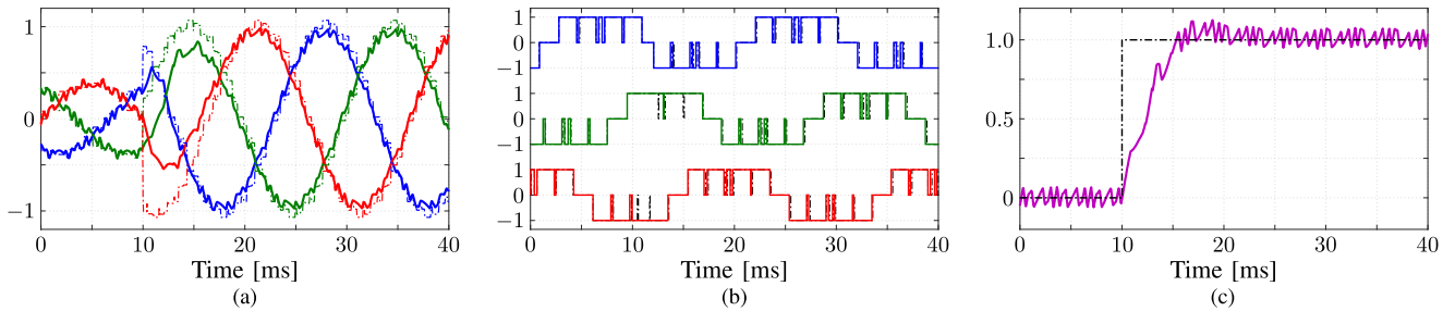
Fig. 11. HIL results produced by the proposed GP 3 C algorithm during a torque reference step-up change. (a) Three-phase stator current i_{s,abc} (solid lines) and their references (dash-dotted lines). (b) Three-phase switching pattern u_{abc} (solid lines) and the nominal OPP (dash-dotted lines). (c) Electromagnetic torque T_e (solid line) and its reference (dash-dotted line).
