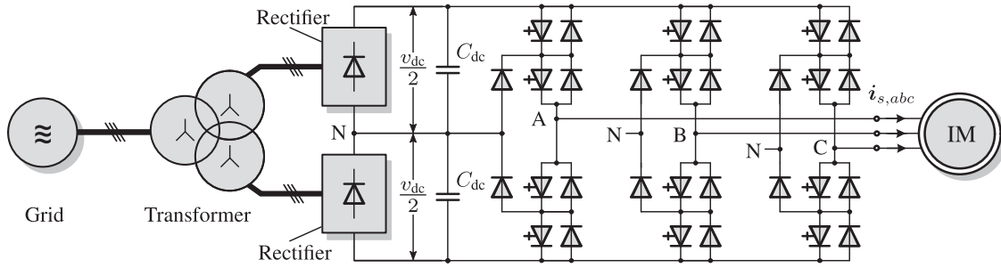
Fig. 1. MV VSD system consisting of a three-level three-phase NPC voltage-source inverter and an induction motor. The inverter has a fixed neutral point potential. The dc link comprises two full-bridge rectifiers connected to the grid via a three-phase transformer.
