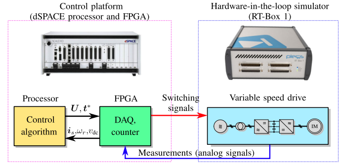
Fig. 3. Block diagram of the HIL test bench.
