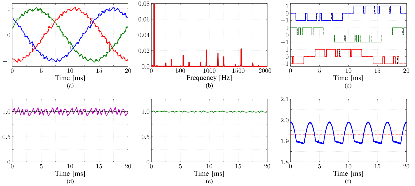
Fig. 6. HIL results of the proposed GP 3 C algorithm at steady-state operation, nominal speed, and rated torque. The modulation index is m = 1.046 , the pulse number d = 5 , and the switching frequency is 250 Hz. (a) Three-phase stator current i_{s,abc} (solid lines) and their references (dash-dotted lines). (a) Stator current spectrum. The TDD is 4.513%. (b) Three-phase switching pattern u_{a,b,c} (solid lines) and the nominal OPP (dash-dotted lines). (c) Electromagnetic torque T_e (solid line) and its reference (dash-dotted line). (d) Stator flux magnitude \Psi_s . (e) Dc-link voltage v_{dc} (solid line) and its average value V_{dc} (dash-dotted line).
