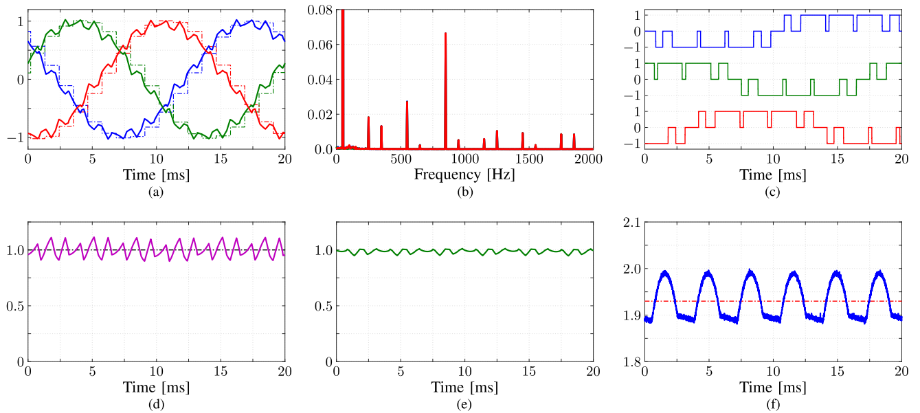
Fig. 7. HIL results of FOC with SVM at steady-state operation, nominal speed, and rated torque. The switching frequency is 250 Hz. (a) Three-phase stator current i_{s,abc} (solid lines) and their references (dash-dotted lines). (b) Stator current spectrum. The TDD is 8.172%. (c) Three-phase switching pattern u_{a,b,c} . (d) Electromagnetic torque T_e (solid line) and its reference (dash-dotted line). (e) Stator flux magnitude \Psi_s . (f) Dc-link voltage v_{dc} (solid line) and its average value V_{dc} (dash-dotted line).
