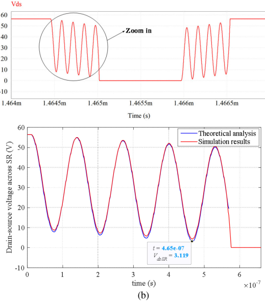
Fig. 9. Comparisons between the simulated results and the theoretical results of the voltage ringing during t_2 – t_3 . (a) With 10 A load current. (b) With 20 A load current.
