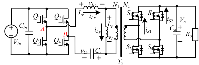
Fig. 1. Full-bridge LLC converter with SR.
