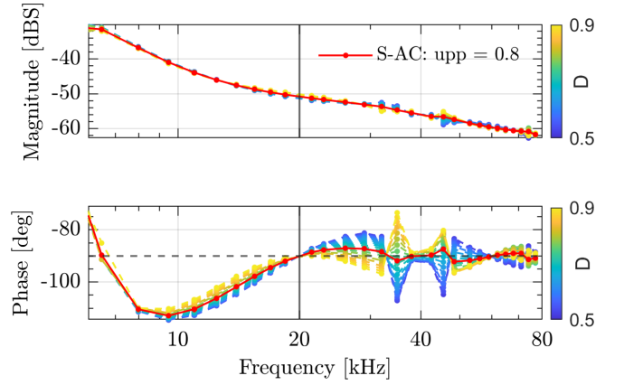
Fig. 3. Comparison between AM during S-ac regime with u_{pp} = 0.8 (red plot) and multiple AMs during SS-dc regimes for the same duty cycle variation range (gradient from blue to yellow). The gray vertical line marks the NF.
