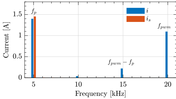
Fig. 15. Comparison between spectra of the current before and after sampling in closed loop operation with 5-kHz perturbation frequency.
