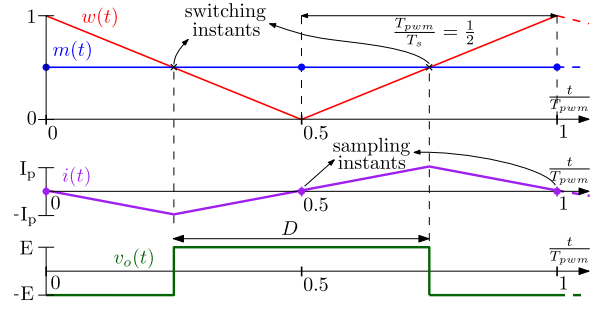
Fig. 2. Synchronization between current sampling instant and switching carrier w to obtain average value of the current i . Sampling is performed at peaks and valleys of w , ideally corresponding to the center of the applied voltage pulse.
