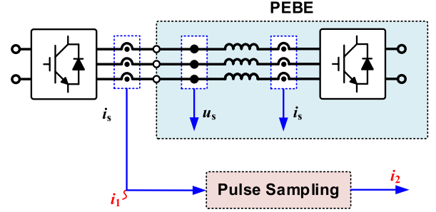
Fig. 17. Analog-to-digital conversion.
