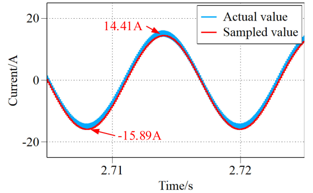
Fig. 18. Waveforms of inductor current when two carriers have the same frequency but mismatched phase. Switching frequency = 10 kHz. Phase difference of carriers = 90^\circ .
