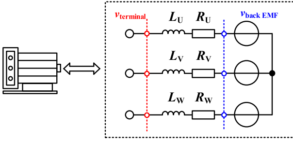
Fig. 5. Terminal voltage and back EMF for emulation of the electric machine.
