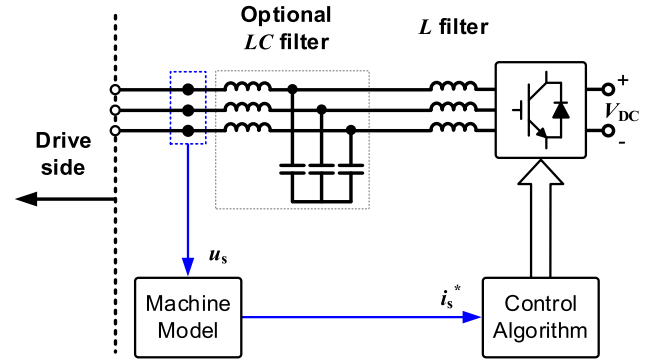
Fig. 7. Open-loop current control.
