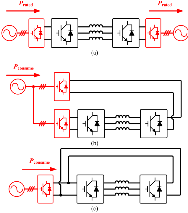
Fig. 14. Power supply solutions for electric machine emulation system. (a) Converters powered by separate power sources. (b) Converters powered by common ac power source. (c) Converters powered by common dc power source.
