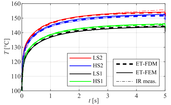
Fig. 8. HB PM temperature response to a current pulse of 57.8 A. Comparison between the proposed ET-FDM approach, the ET-FEM model, and IR measurements.
