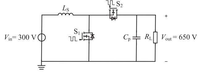
Fig. 10. Circuit schematic of the simulated 100-kHz synchronous boost converter with the output power P_{out} = 13.5 kW, the dead time t_{dead} = 200 ns, input voltage V_{in} = 300 V, and output voltage V_{in} = 650 V. S1 and S2 are 1.2-kV 40-mΩ SiC MOSFETs.
