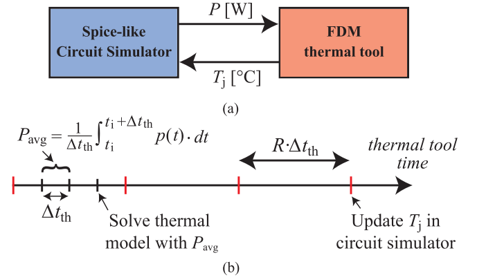
Fig. 7. Coupling of the proposed FDM thermal tool with a commercial circuit simulator. (a) Data transfer between the tools. (b) Example of time steps for the proposed FDM thermal tool; T_j is updated in the circuit netlist every R \cdot \Delta t_{th} .
