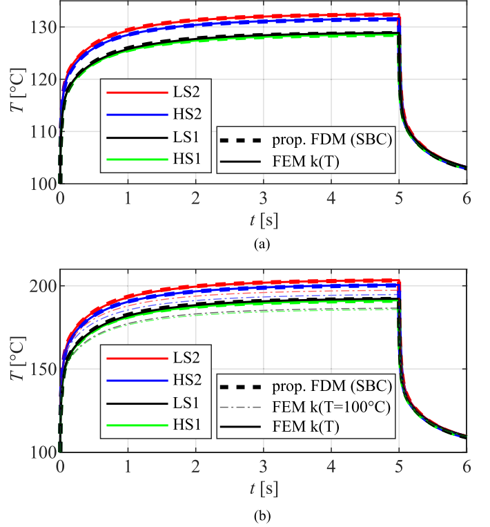
Fig. 5. Comparison of the proposed FDM-SBC approach with a commercial FEM tool, power pulse response of the HB PM (see Fig. 2) for (a) 50 W and (b) 150 W applied to the four dies. In (b), the response for k(T = 100^\circ\text{C}) is shown for comparison.
