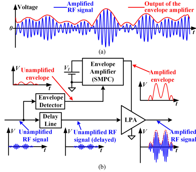
Fig. 1. Overview of an ET system. (a) Key waveforms. (b) General scheme.
