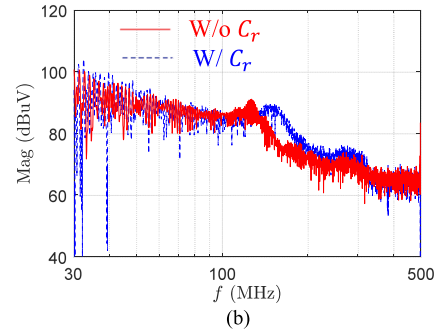
Fig. 20. V_{SW} before and after C_r is added. (a) Waveform. (b) Spectra.
