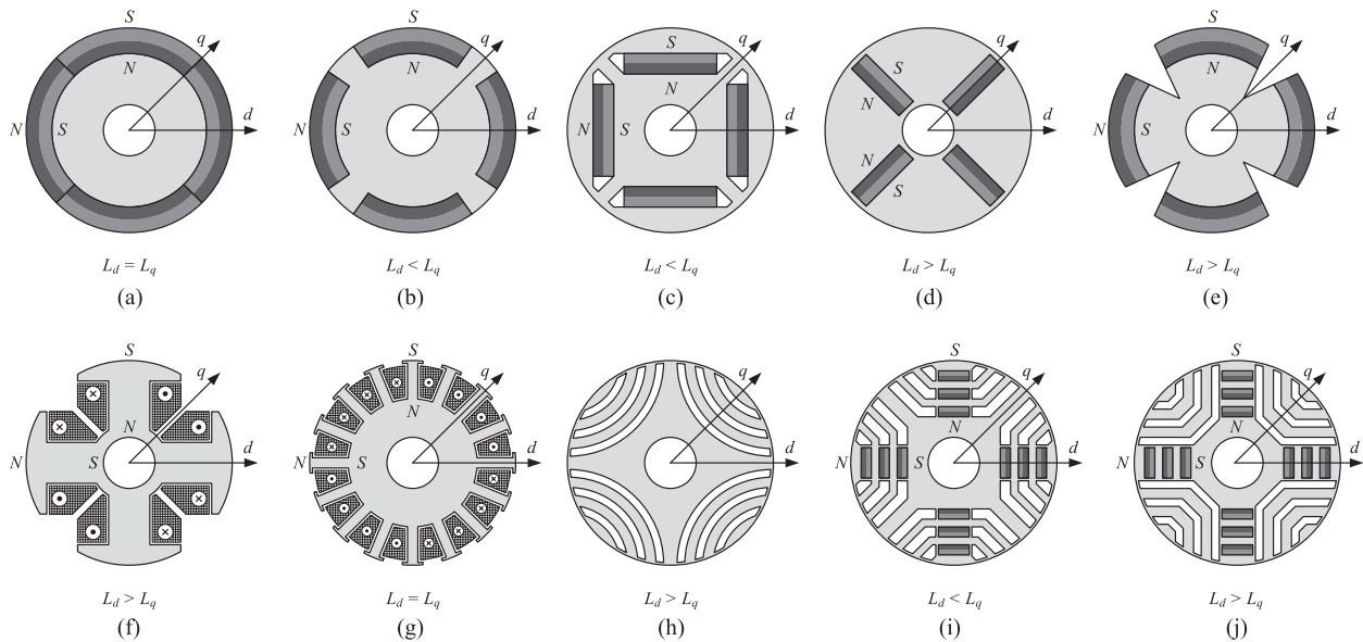
Fig. 1. Design of the most popular synchronous motors: (a) surface mounted magnets, (b) inset magnets, (c) interior tangential magnets, (d) interior radial magnets, (e) pole salient with magnets, (f) pole salient wound rotor, (g) nonpole salient wound rotor, (h) synchronous reluctance, (i) and (j) PM assisted synchronous reluctance.
