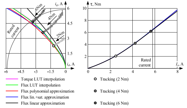
Fig. 8. Comparison of MTPA tracking and offline MTPA trajectories based on torque measurements, flux measurements, or flux maps approximations.
