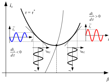
Fig. 9. Small-signal approach for MTPA tracking according to the “LF” injection method.
