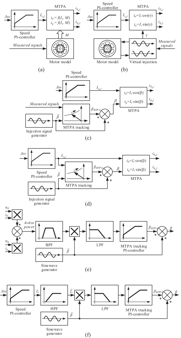
Fig. 6. Modifications of the conventional control scheme for implementation of MTPA online methods. (a) Parameters estimation. (b) Virtual signal injection. (c) and (e) High-frequency injection. (d) and (f) Low-frequency injection.
