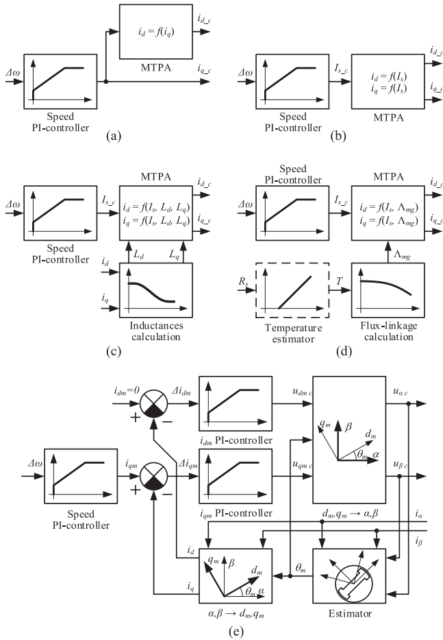
Fig. 5. Modifications of the conventional control scheme for implementation of MTPA offline methods. (a) and (b) Analytical approach. (c) Inductance calculation as a function of current. (d) Flux-linkage calculation as a function of temperature. (e) Motor parameters calculation in the MTC reference frame.
