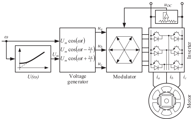
Fig. 7. Conventional SC scheme.
