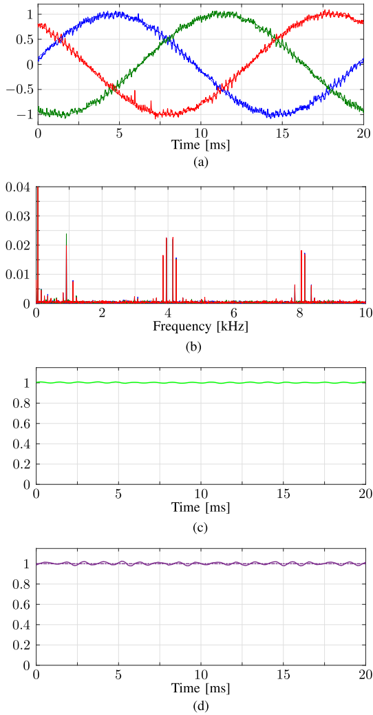
Fig. 9. Experimental results of FOC at steady-state operation, f_{sw} = 4050 Hz. (a) Three-phase stator current i_{s,abc} . (b) Stator current harmonic spectrum. The THD is 6.18%. (c) Stator flux magnitude \Psi_s . (d) Electromagnetic torque T_e .
