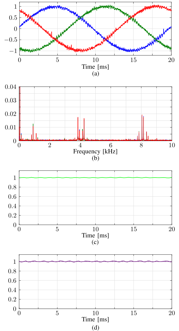
Fig. 8. Experimental results of direct MPC at steady-state operation, f_{\text{sw}} = 4050 Hz. (a) Three-phase stator current i_{s,abc} . (b) Stator current harmonic spectrum. The THD is 5.80%. (c) Stator flux magnitude \Psi_s . (d) Electromagnetic torque T_e .
