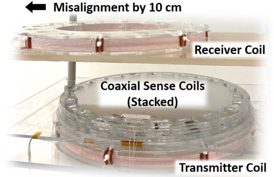
Fig. 37. FC-TPM was demonstrated over Rx coil misalignment when coaxially stacked sense coils were used.
