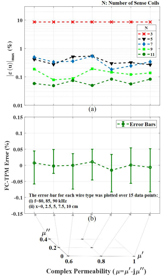
Fig. 20. (a) Worst-case absolute error percentage for each type of wire (represented by the complex permeability) as the number of sense coils is increased. (b) The spread in error using 11 sense coils for each type of wire over both frequency and misalignment variation.
