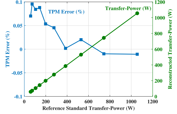
Fig. 32. FC-TPM was demonstrated in hardware over a wide range of power levels.
