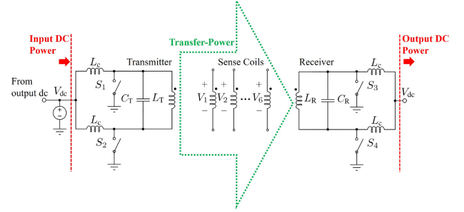
Fig. 25. Current-mode class D wireless power transfer system with open-circuited FC-TPM sense coils. DC current was recirculated with the input and output voltage held fixed.
