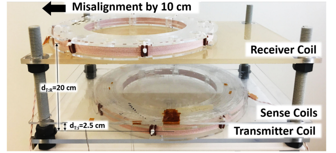
Fig. 33. Faraday coil transfer-power measurement was demonstrated over SAE J2954 Rx coil misalignment.
