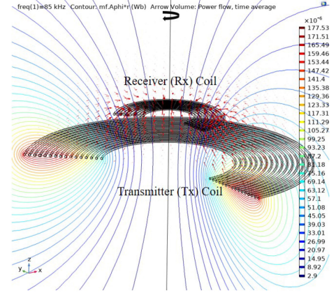
Fig. 41. Multiturn concentric solid wires were used for the Tx and Rx coils to emulate WPT2/Z1 class.
