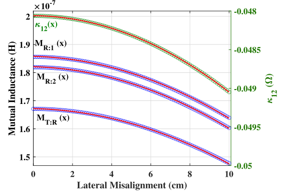
Fig. 13. Numerical results of the relevant mutual inductances (blue-dots): 1) Tx-to-Rx; and 2) Rx-to-sense-coils. The geometric parameter \kappa_{12}(x) (green-dots) in (45) for two coplanar sense coils (sense coil 1 and 2, specified in Table II) are plotted over Rx coil misalignment. Red lines are the corresponding second-order polynomial fits.
