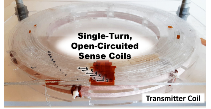
Fig. 24. Sense coils are in the flat plane above the Tx coil.
