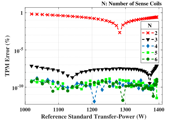
Fig. 17. FEM simulation was performed to show FC-TPM errors when eddy currents in the Tx and Rx coils are included.
