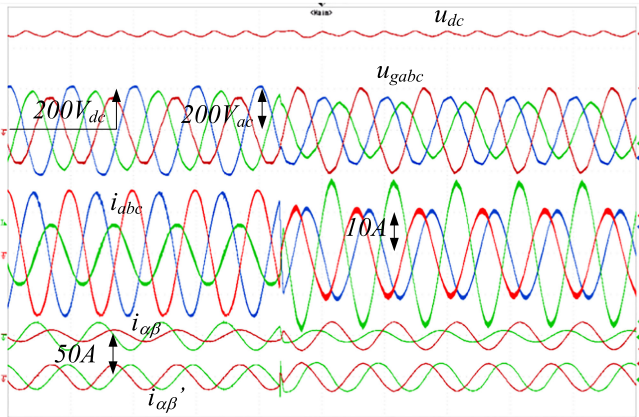
Fig. 12. Experimental results of step response of current control loop to arbitrarily changed reference current imbalance ( u_{dc} – dc bus voltage, u_{sabc} – three-phase grid voltage, i_{abc} – three-phase converter current, i_{\alpha\beta} – converter current components in the natural stationary frame, i_{\alpha\beta}' – converter current components in a new stationary frame).
