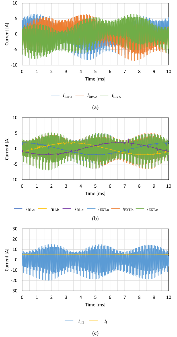
Fig. 16. Time-domain waveforms m_a = 0.5 , k_7 = 0.0 , and \alpha = 0^\circ . (a) Inverter currents. (b) Three-phase load currents & extraction circuit currents. (c) Transformer primary side current and auxiliary load current.
