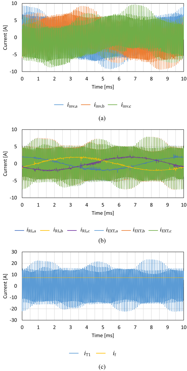
Fig. 15. Time-domain waveforms m_a = 0.5 , k_7 = 0.5 , and \alpha = 0^\circ (a) Inverter currents. (b) Three-phase load currents & extraction circuit currents. (c) Transformer primary side current and auxiliary load current.
