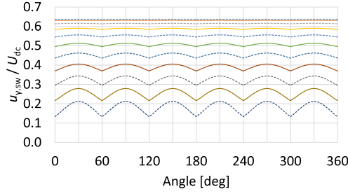
Fig. 5. Switching harmonics in each switching cycle ( k_7 = 0 and \alpha = 0^\circ ).
