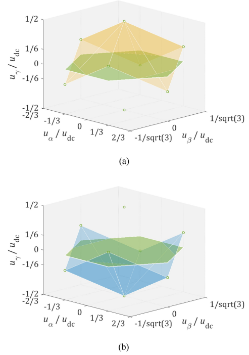
Fig. 4. SVM switching states in \alpha\beta\gamma -frame (a) Upper three rhombi and SVM hexagon. (b) Lower three rhombi & SVM hexagon.
