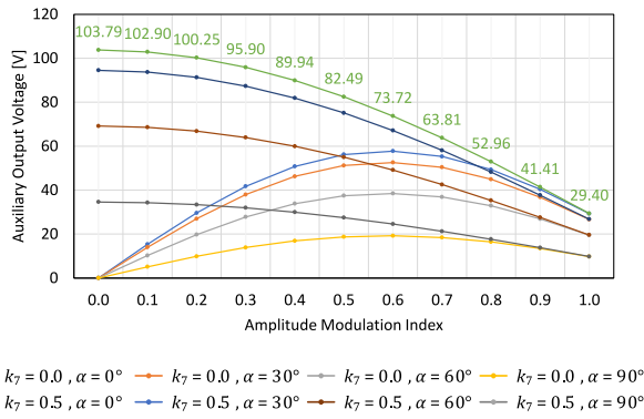
Fig. 12. Auxiliary voltage output in from theoretical calculations.
