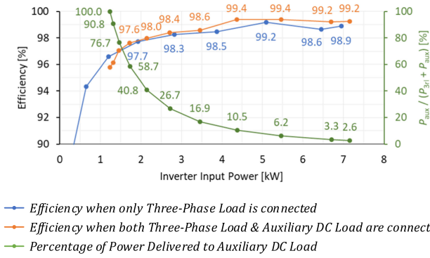
Fig. 18. Experimental comparison of inverter efficiency between the cases with and without the auxiliary dc load.
