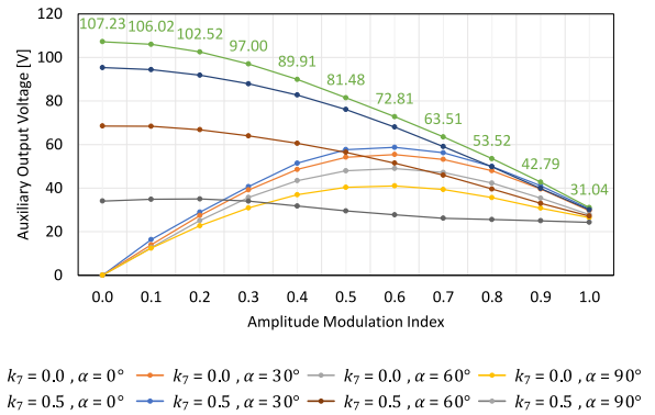
Fig. 13. Auxiliary voltage output in circuit simulations.
