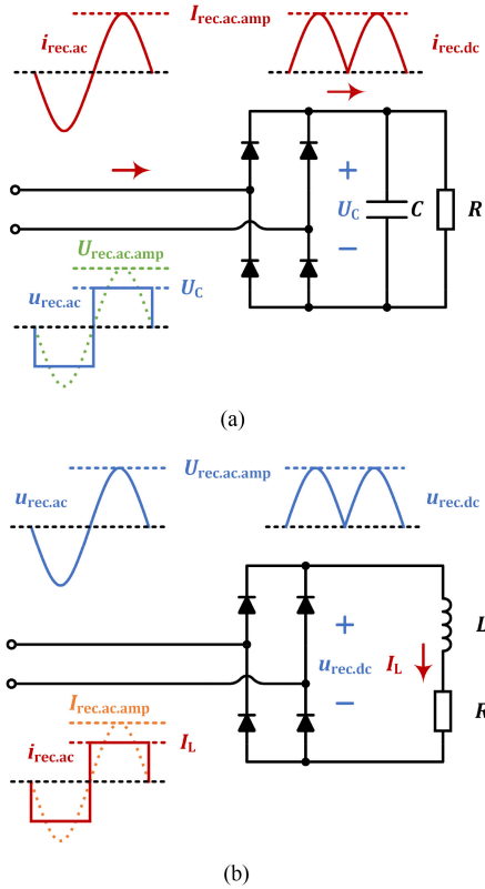
Fig. 9. Rectifier connected with capacitive or inductive load. (a) Rectifier and capacitive load. (b) Rectifier and inductive load.
