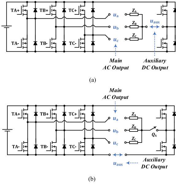
Fig. 1. Schematic diagrams of the circuits proposed in previous studies which utilize the neutral point of the three-phase load to extract common mode switching harmonics for auxiliary power output. (a) Schematic diagram of the circuit proposed in [12]. (b) Schematic diagram of the circuit proposed in [13] and evaluated in [14].
