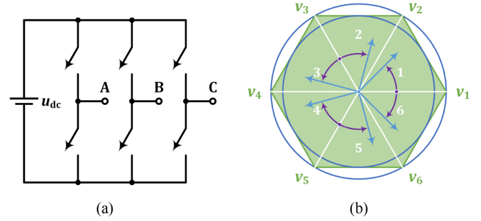
Fig. 3. Three-phase inverter with SVM. (a) Three-phase inverter. (b) SVM hexagon on \alpha\beta -plane.
