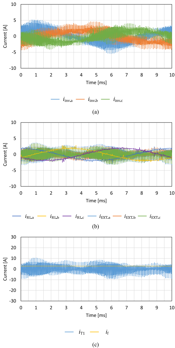
Fig. 17. Time-domain waveforms m_a = 0.5 , k_7 = 0.5 , and \alpha = 90^\circ . (a) Inverter currents. (b) Three-phase load currents and extraction circuit currents. (c) Transformer primary side current and auxiliary load current.
