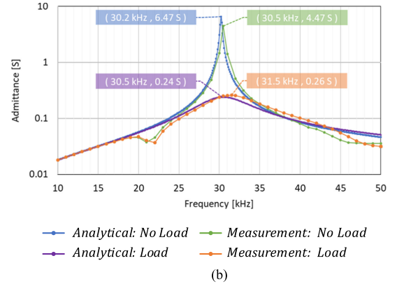
Fig. 11. Resonance analysis. (a) Diagram of resonance circuit. (b) Admittance of the resonance circuit.
