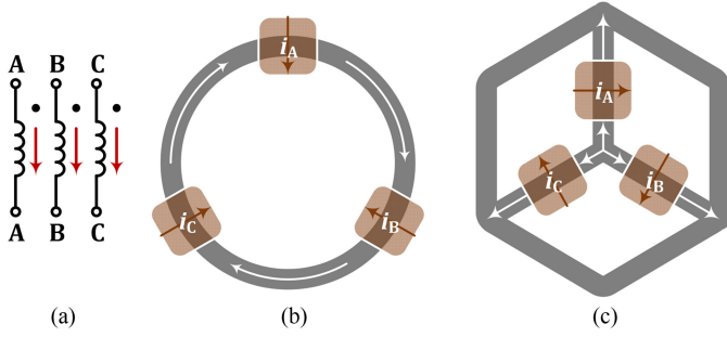
Fig. 7. DM- and CM-passing coils. (a) Reference direction of currents. (b) DM-Passing coil. (c) CM-Passing coil.
