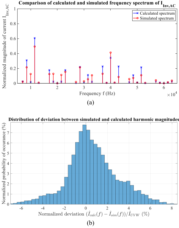
Fig. 7. (a) Comparison of the calculated and simulated frequency spectrum of I_{Inv,AC} for the following operating point: I_{UVW} = I_{RST} = 1A , f_{f1} = f_{f2} = 500 Hz, \cos(\varphi_1) = \cos(\varphi_2) = 0.6 , \beta = 8\pi/5 , M_1 = M_2 = 0.9 , \sigma = \pi/2 . (b) Normalized deviation (\hat{I}_{calc}(f) - \hat{I}_{sim}(f)) / \hat{I}_{UVW} for six harmonic frequencies ( f \in \{f_{sw}; 3 \cdot f_f + f_{sw}; 2 \cdot f_{sw}; 6 \cdot f_f + 2 \cdot f_{sw}; 3 \cdot f_{sw}; 3 \cdot f_f + 3 \cdot f_{sw}\} ) of 5^6 operating points.
