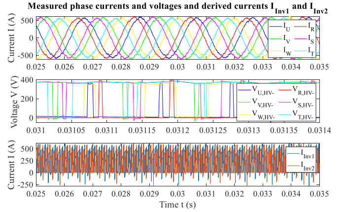
Fig. 10. Measured signals for an exemplary operating point and derived dc-link currents of the two subinverters. \hat{I}_{\text{UVW}} \approx \hat{I}_{\text{RST}} \approx 590 A, f_{f1} \approx f_{f2} = 500 Hz, \cos(\varphi_1) = 0.58 , \cos(\varphi_2) = 0.56 , \beta = 5.55 , M_1 \approx M_2 \approx 0.89 , \sigma = \frac{\pi}{2} ; T = 100 N·m.
