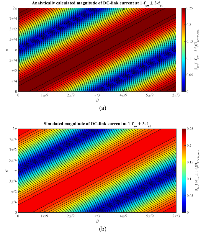
Fig. 6. Magnitude of I_{Zk}(f) at f = f_{sw} \pm 3 \cdot f_f as a function of \sigma and \beta . Considered operating point: I_{UVW} = I_{RST} , M_1 = M_2 = 0.5 , \varphi_1 = \varphi_2 = \pi/3 , f_{f1} = f_{f2} = 200 Hz. (a) Analytically calculated. (b) Simulated.
