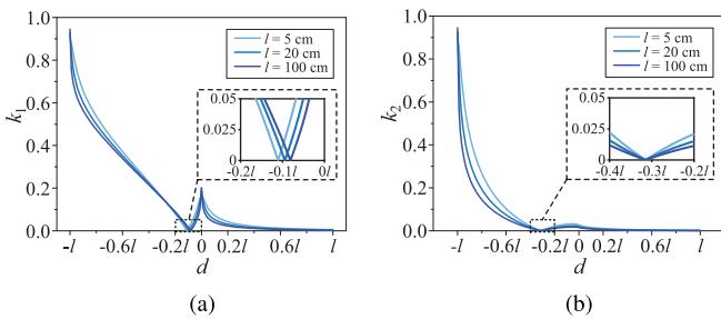
Fig. 6. Cross coupling coefficients versus different d and l . (a) k_1 . (b) k_2 .
