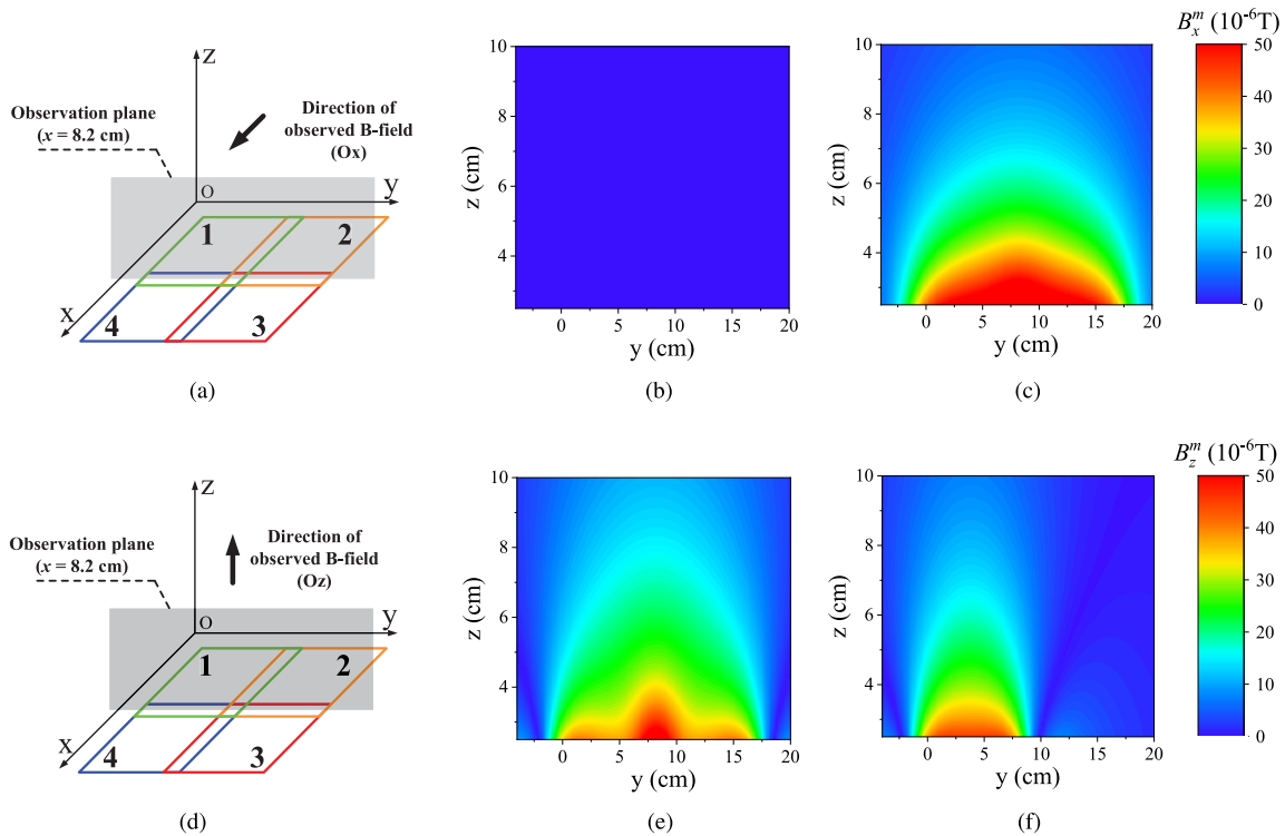
Fig. 10. Calculation results of B-field ADFs generated by a 2 \times 2 planar Tx-coil array ( x = 8.2 cm). (a) Layout and coordinates for Fig. 10(b) and (c). (b) \theta_1 = 0^\circ , \theta_2 = 0^\circ , \theta_3 = 0^\circ , and \theta_4 = 0^\circ . (c) \theta_1 = 0^\circ , \theta_2 = 0^\circ , \theta_3 = 180^\circ , and \theta_4 = 180^\circ . (d) Layout and coordinates for Fig. 10(e) and (f). (e) \theta_1 = 0^\circ , \theta_2 = 0^\circ , \theta_3 = 0^\circ , and \theta_4 = 0^\circ . (f) \theta_1 = 0^\circ , \theta_2 = 0^\circ , \theta_3 = 180^\circ , and \theta_4 = 0^\circ .
