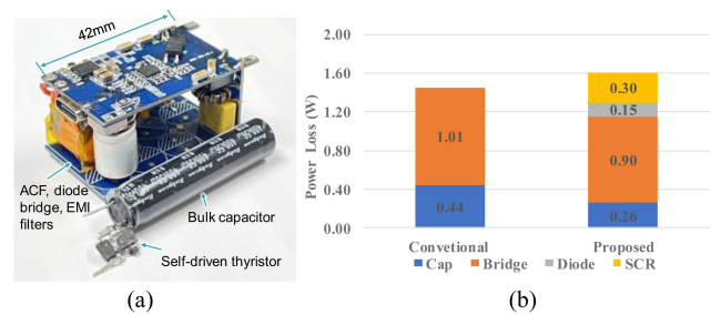
Fig. 8. (a) Prototype used to verify the proposed method for bulk capacitance reduction in the rectifier for a GaN-based ACF converter. (b) Rectifier loss breakdown comparison between conventional and proposed methods.
