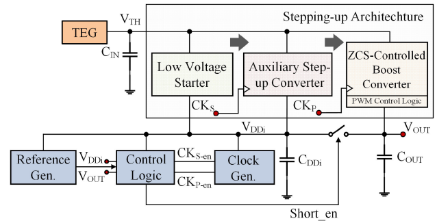
Fig. 11. Single-stage SISO step-up converter as a TEG energy harvesting interface proposed in [130].
