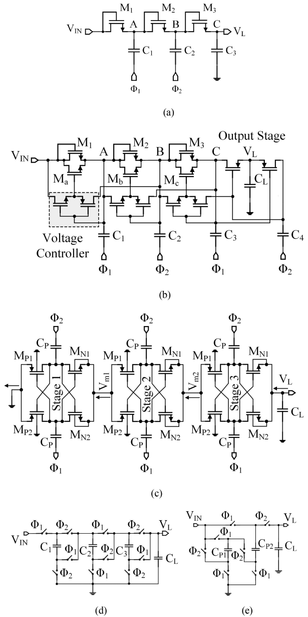
Fig. 17. Schematics of different SC topologies. (a) Conventional Dickson CP [155]. (b) Modified Dickson CP used in [6]. (c) Pelliconi architecture based three-stage negative charge pump used in [16]. (d) Fibonacci 5:1 SC network used in [154]. (e) Series–parallel SC topology used in [7].
