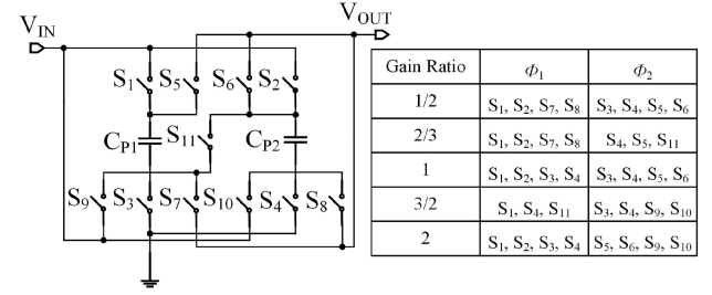
Fig. 18. Five-GR reconfigurable SC converter power stage along with its different switching schemes [151].
