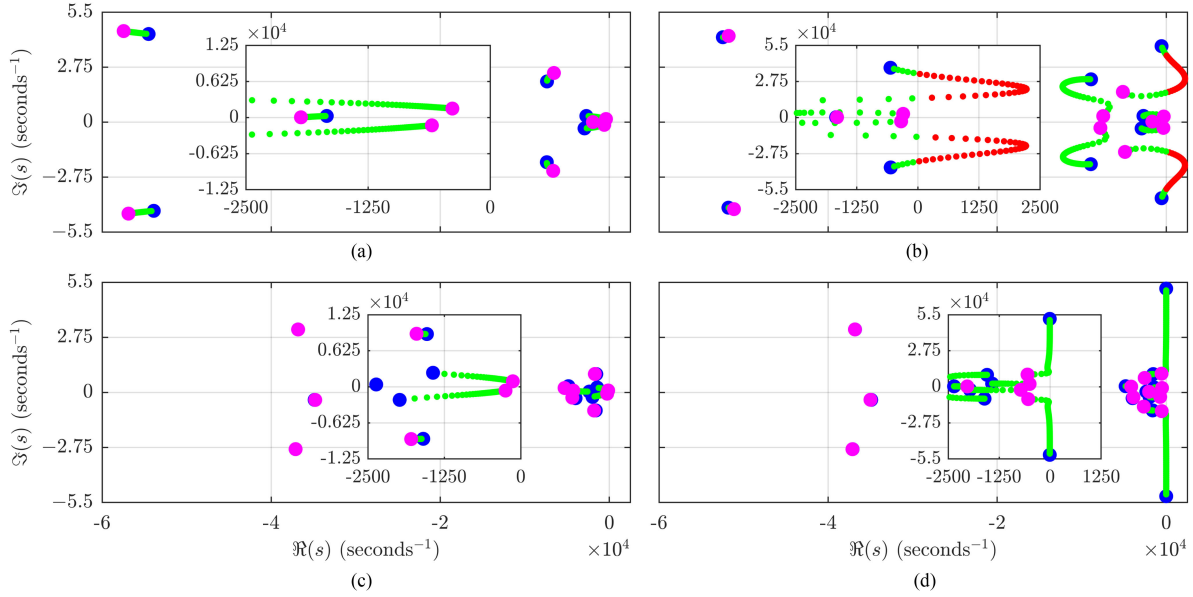
Fig. 12. Pole map evolution of [I + \mathbf{Y}\mathbf{Z}_g] = 0 , being \mathbf{Z}_g L -type, where L_g \in [0.425, 4.25] mH, or LC -type, where L_g = 0.425 mH and C_g \in [2.38 \text{ } 238] \mu\text{F} (from blue to magenta). Cases and type of \mathbf{Z}_g . (a) L^{c1} and L -type. (b) L^{c1} and LC -type. (c) LCL and L -type. (d) LCL and LC -type.
