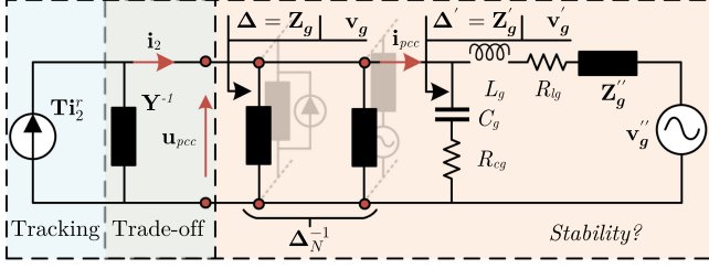
Fig. 5. Current-controlled VSC facing PCC uncertainty (from left to right): several paralleled VSCs with equivalent admittance identified as \Delta_N ; LC-type cable model; remaining grid given by Z_g'' and voltage v_g .
