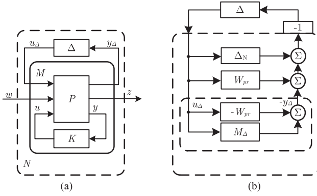
Fig. 2. (a) M - \Delta structure for robust stability analysis. (b) Model modification for PBRC assessment when \Delta is passive and the system to be controlled M_\Delta is paralleled with another uncertain system \Delta_N with a passivity shortage.
