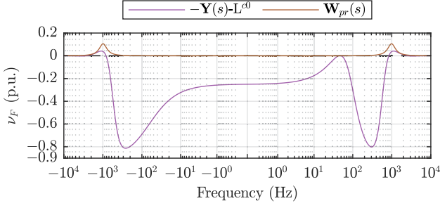
Fig. 7. IFP of -Y in case L^{c0} and W_{pr} for PBRC assessment.
