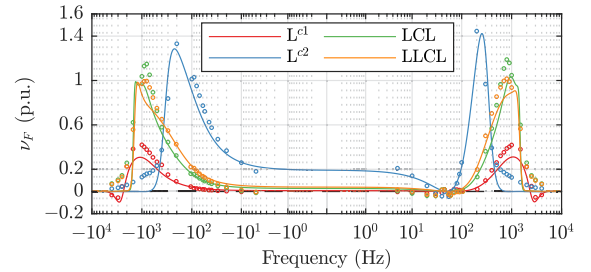
Fig. 15. Experimental input admittance IFP index with circle markers (o) compared with its corresponding theoretical one in solid line.
