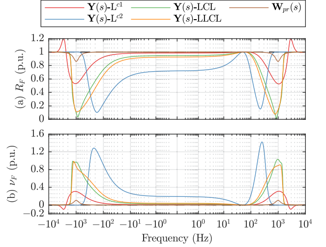
Fig. 8. Passivity indices of Y for each case under study. (a) R -index R_F . (b) IFP index \nu_F .
