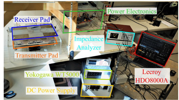
Fig. 11. Test-rig and testing equipment.
