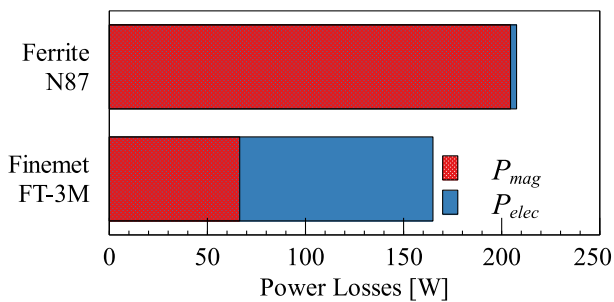
Fig. 10. Estimation of core losses with ferrite and nanocrystalline ribbon cores at 6.6 kW.
