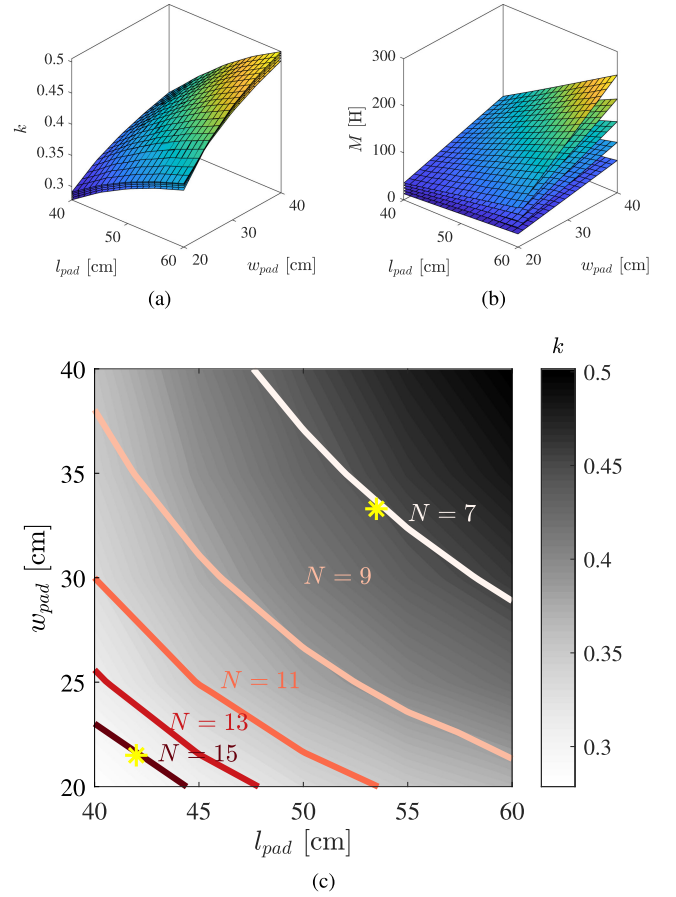
Fig. 6. Design space for the WPT3/Z1 (11 kW). l_{pad} , w_{pad} , and N versus (a) k . (b) M . The contour lines in (c) define the pad size required to obtain the target mutual inductance of 64 \mu\text{H} . *: selected designs.
