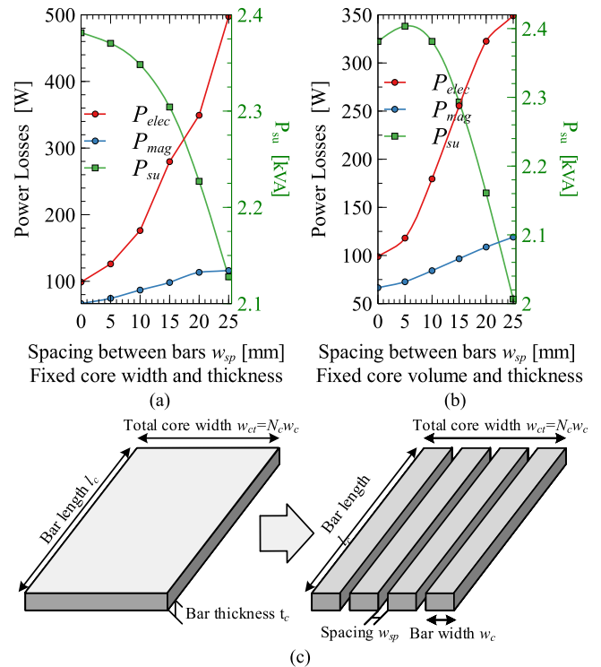
Fig. 8. Analysis of the spacing between bars on the power transfer capability of the pad P_{su} , eddy-current losses P_{elec} , and hysteresis losses P_{mag} . In (a) the core width is constant while in (b) the core volume is constant. The core thickness ( t_c ) is constant at 4 mm is constant. (c) Definition of terms. i_{1,pk} = 21 A.
