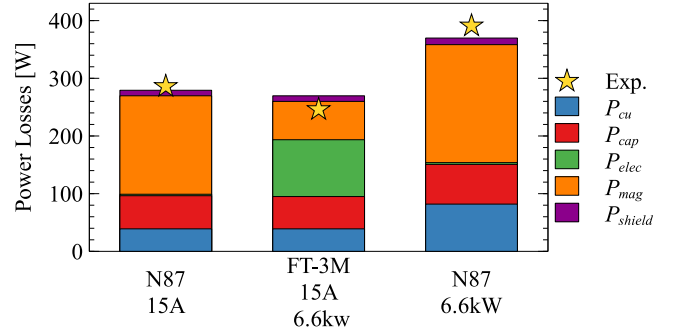
Fig. 15. Breakdown of losses in the pads with N87 and Finemet FT-3 M cores. The losses are compared at the same current and the same power.
