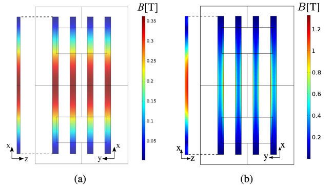
Fig. 3. Flux density distribution for (a) N87 and (b) nanocrystalline core bars at an air gap of 100 mm. Result obtained from [9].
