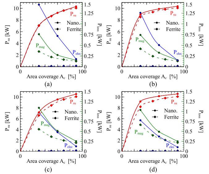
Fig. 5. Power transfer capability/uncompensated power P_{su} , eddy-current losses P_{elec} , and hysteresis losses P_{mag} , for a double-D pad nanocrystalline ribbon and ferrite cores. The x -axis depicts the percentage of the pad's surface area covered by core material (area coverage). Different core thicknesses t_c and number of cores N_c are tested. i_{1,rms} = 23 A. (a) N_c = 4 t_c = 12 mm. (b) N_c = 8 t_c = 12 mm. (c) N_c = 4 t_c = 8 mm. (d) N_c = 8 t_c = 8 mm.
