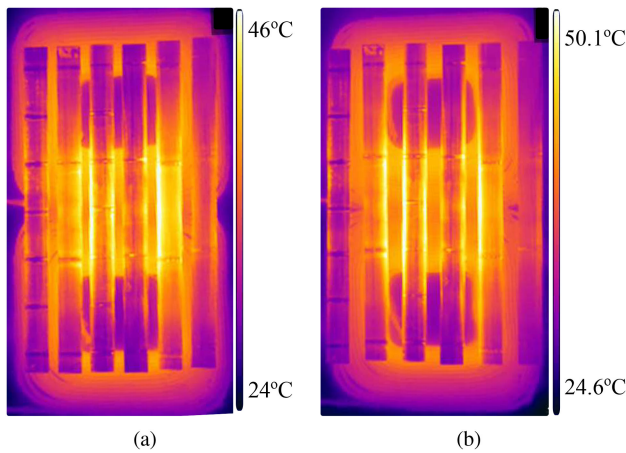
Fig. 23. Temperature distribution of the cores after operation at 3.3 kW for 5 min. Separation between cores: (a) 10 mm and (b) 15 mm.
