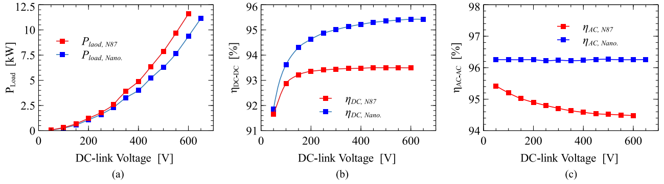
Fig. 14. Power loss measurement for double-D pad with N87 cores and Nanocrystalline cores. (a) Output power to the load. (b) Overall efficiency of the system \eta_{DC-DC} . (c) Efficiency of the pad without considering the power converters.
