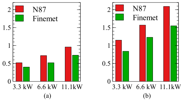
Fig. 16. Measured leakage flux at 800 mm from the center of the pad. The mid-plane between Tx and Rx is considered. Two points are selected. (a) One parallel to y -axis and another one parallel to the (b) x -axis. Axes are defined in Fig. 2.
