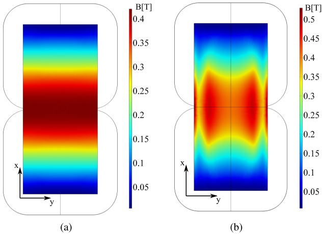
Fig. 9. Flux density distribution within the core using (a) ferrite N87 and (b) finemet FT-3 M cores. Air gap: 100 mm. I_{pk} = 40 A.
