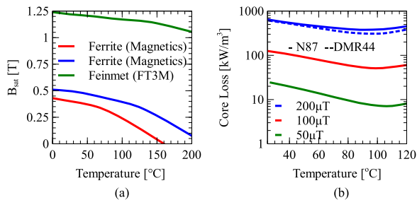
Fig. 19. (a) Saturation flux density for nanocrystalline ribbon FT-3M [18], and MnZn ferrites [24] versus temperature. (b) Core losses versus temperature for different MnZn ferrites: N87 and DMR44.
