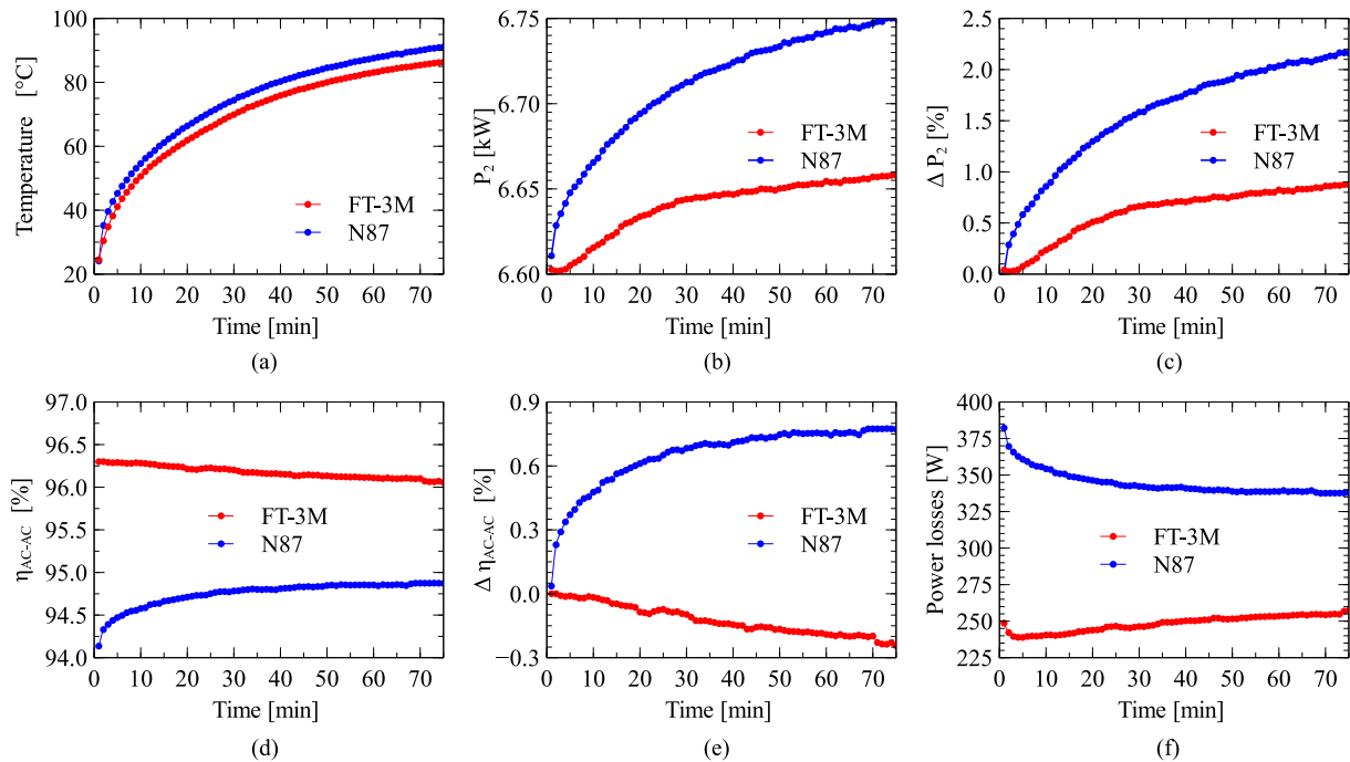
Fig. 21. Pad performance versus time/temperature. (a) Measurement of the temperature at the center of the core. (b) Power transfer and (c) its variation versus time/temperature. (d) Pad's efficiency and (e) its variation versus time/temperature. (f) Power losses.
