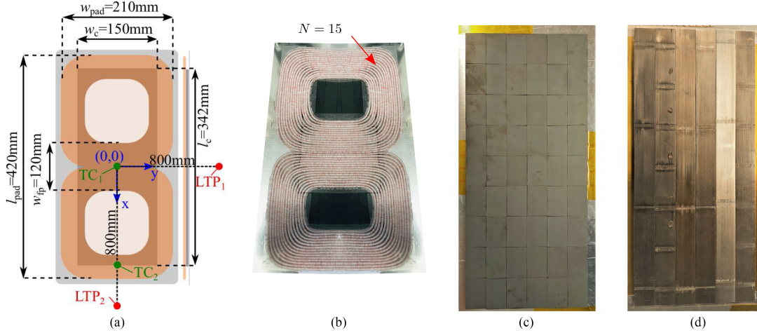
Fig. 12. (a) Double-D pad's dimensions. LTP: leakage flux test-point. TC: thermo-couple location. (b) Depiction of the constructed pad. (c) Ferrite core. (d) Finemet FT-3 M nanocrystalline ribbon core.
