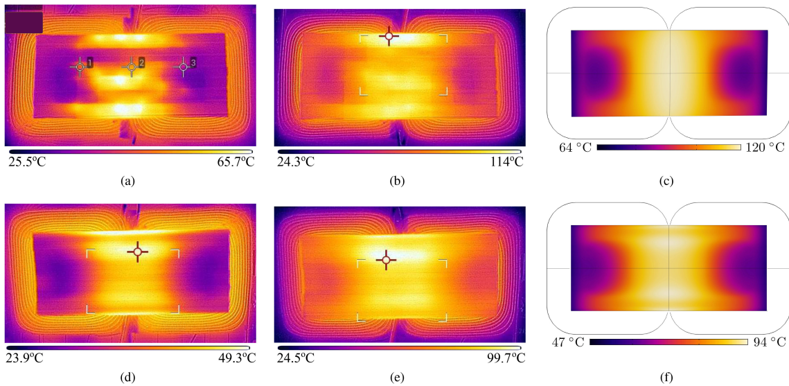
Fig. 20. Temperature distribution of the cores at 6.6 kW. (a)–(c) correspond to the ferrite cores (tiles). (d)–(f) correspond to the nanocrystalline ribbon cores. (a), (d) Temperature distribution after a 5 min operation. (b), (e) Temperature distribution at thermal equilibrium. (c), (f) Simulation results at thermal equilibrium.
