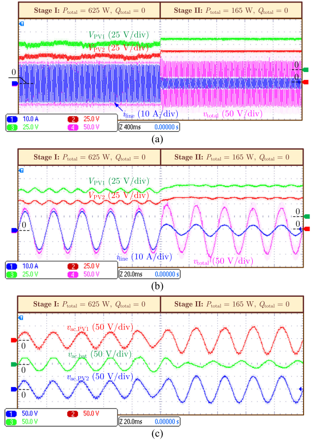
Fig. 14. Voltage and current response of the series PVBH system during load active power step change: (a) PV voltages, grid voltage, and current, (b) zoomed-in plot of (a), and (c) output voltages of the three converters.
