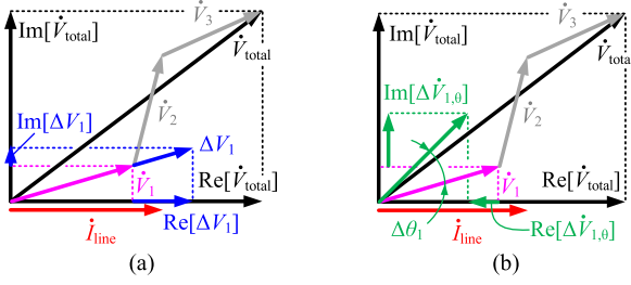
Fig. 2. Phasor diagram of a 3-cell series system shown in Fig. 1 when (a) output voltage amplitude of converter #1 varies, and (b) phase angle of converter #1 varies.
