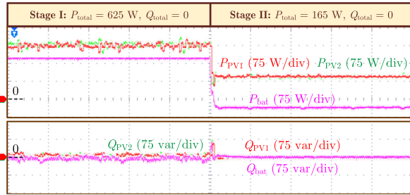
Fig. 13. Power control performance of the series PVBH system during load active power step change.
