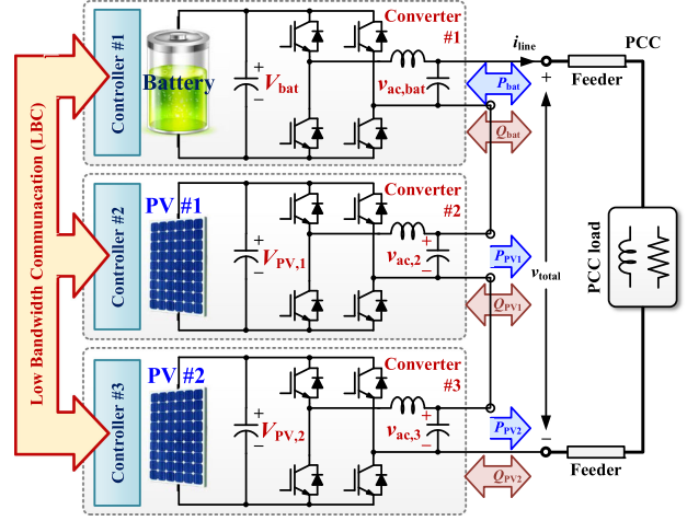
Fig. 1. Hardware schematic of a 3-cell series PVBH system, where v_{ac,k} and v_{ac,bat} are the ac voltages of the k th converter cell and the battery cell, respectively, V_{PV,m} and V_{bat} are the dc voltages of PV # m and the battery, respectively, and v_{total} is the output voltage of the system.
