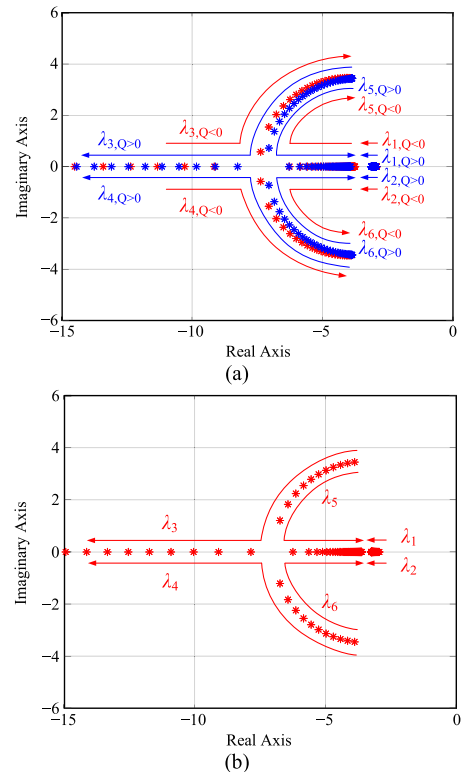
Fig. 8. Root loci diagrams for the islanded system when steady states varies. (a) V_{total} changes from 296 to 326 V. (b) \theta_{total} changes from 0.02 to 0.12 rad.
