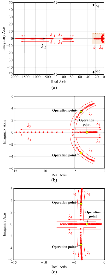
Fig. 6. Root loci diagrams for the islanded system when the control parameters of PV converters vary: (a) k_{p,p} and k_{p,q} for all PV converters change from 0.06 to 0.3, (b) zoomed-in plot of Fig. 6(a), and (c) zoomed-in diagram when k_{i,p} and k_{i,q} for all PV converters change from 0.08 to 0.8.
