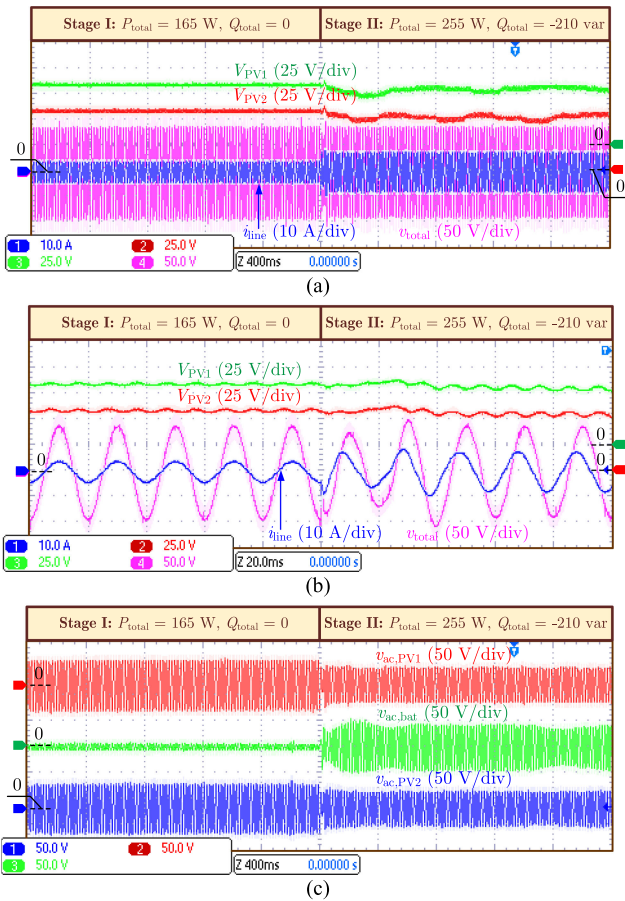
Fig. 19. Voltage and current response of the series PVBH system during load active and reactive power change when PV power is halved: (a) PV voltages, grid voltage and current; (b) zoomed-in plot of (a); and (c) output voltages of the three converters.
