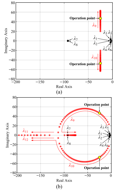
Fig. 7. Root loci diagrams for the islanded system when the control parameters of the battery converter vary. (a) k_{D,p} changes from 2.28 \times 10^{-5} to 1.03 \times 10^{-4} rad/(W·s). (b) \omega_{cut,total} changes from 10 to 300 rad/s.
