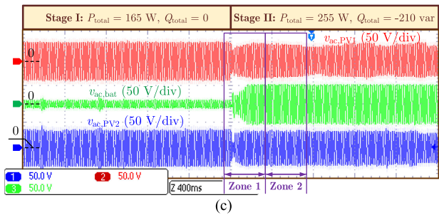
Fig. 16. Voltage and current response of the series PVBH system during load active and reactive power change: (a) PV voltages, grid voltage, and current, (b) zoomed-in plot of (a), and (c) output voltages of the three converters.
