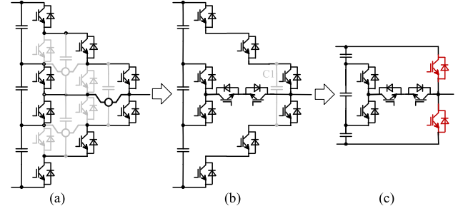
Fig. 7. Derivation of a new four-level converter topology.
