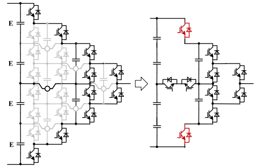
Fig. 11. Five-level topology derived from the generalized topology.
