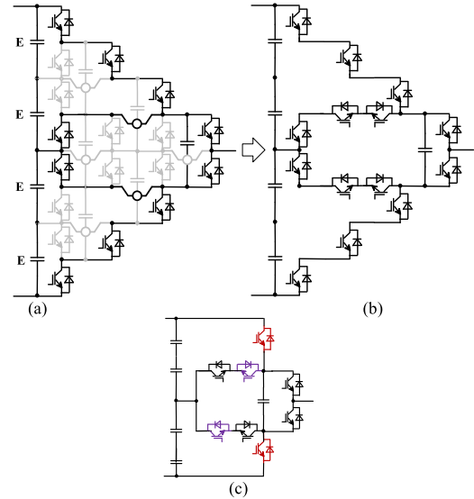
Fig. 12. Five-level converter topology.
