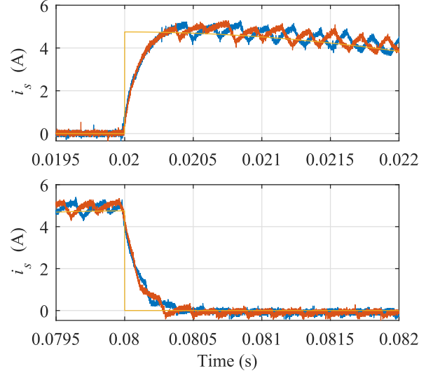
Fig. 17. Zoom-in views of the ac-side current dynamic responses of the wired (blue), wireless (orange) cases, and i_s^* (yellow) around the step times. At 0.02 s, i_s^* is stepped from 0 to 4.75 A and at 0.08 s, back to 0 A.
