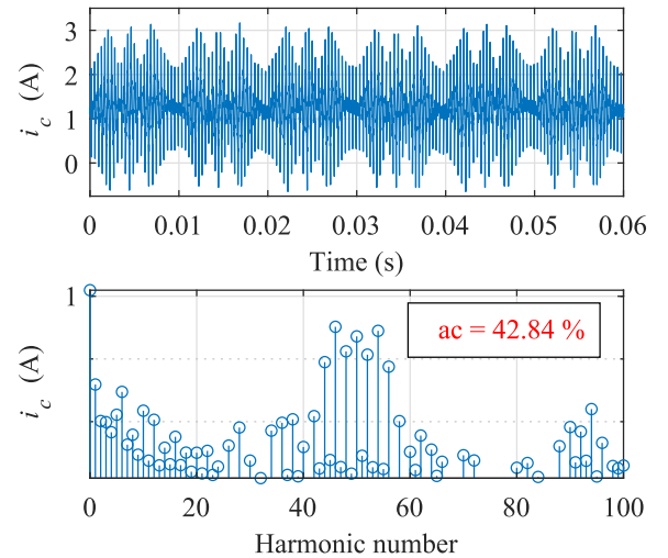
Fig. 14. Circulating current (upper) and harmonics spectrum (lower). The ac value corresponds to I_{ac,rms}/I_{dc} , including all the ac harmonics. DC is 1.25 A.
