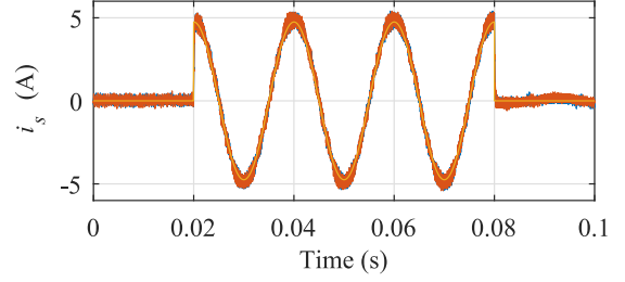
Fig. 16. AC-side current dynamic responses of the wired (blue), wireless (orange) cases, and i_s^* (yellow) overlapped. At 0.02 s, i_s^* is stepped from 0 to 4.75 A and at 0.08 s, back to 0 A.
