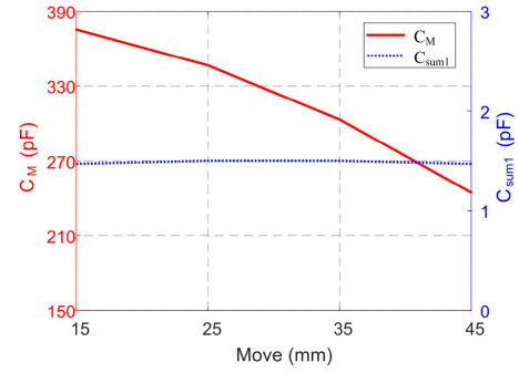
Fig. 13. Variation of capacitances C_M and C_{\text{sum}1} regarding movement.
