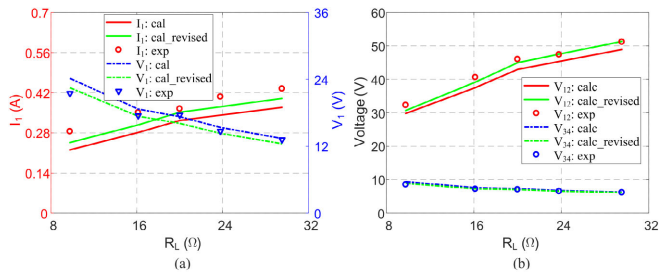
Fig. 23. Experimental, calculated, and revised-calculated (a) input current I_1 and input voltage V_1 , and (b) voltage V_{12} across the transmitting plates and voltage V_{34} across the metal cover at different load resistance R_L .
