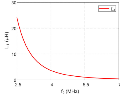
Fig. 14. Variation of inductance L_1 as a function of operating frequency when Move = 45 mm.
